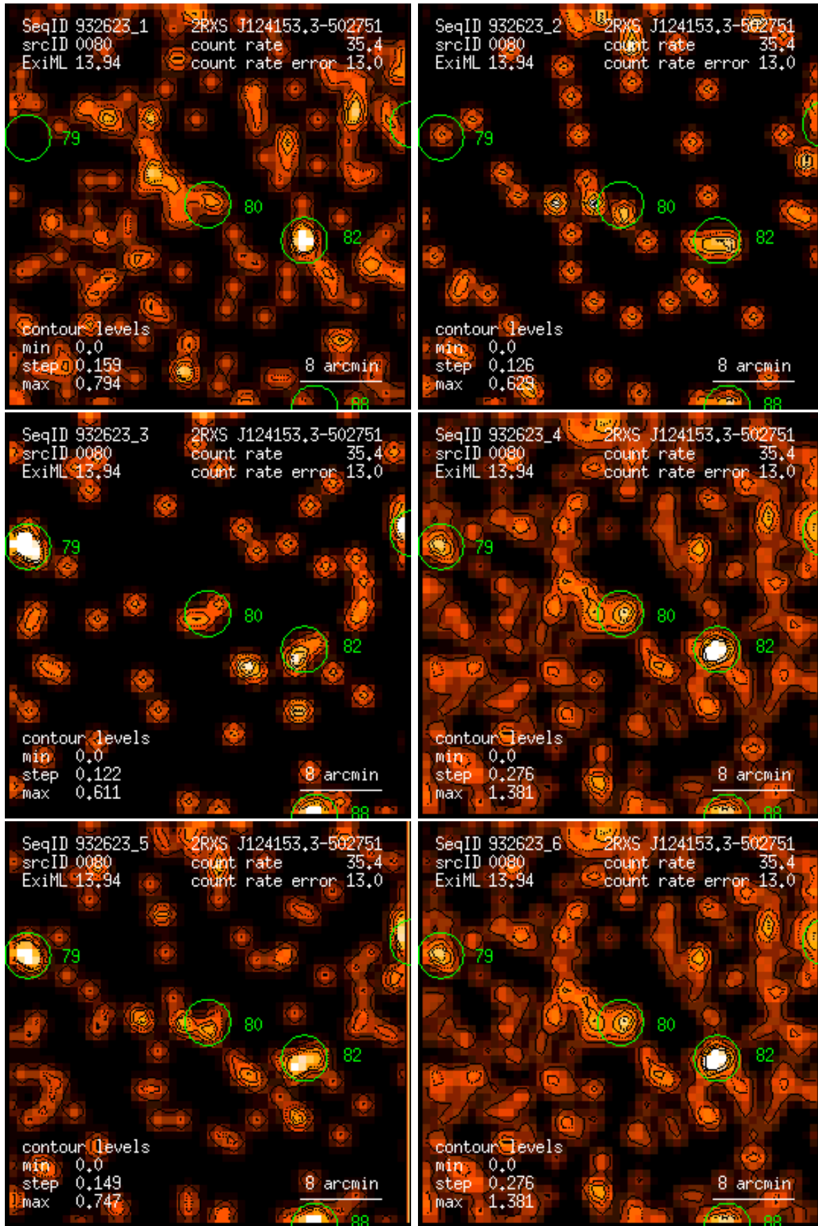
Figure 80: RASS 932623: detection 0080: band rate images, Gaussian filter: (1) PSPC channels 11 – 41, (2) 52 – 90, (3) 91 – 201, (4) 11 – 235, (5) 52 – 201, (6) 11 – 201. Broad band rates in counts/ks. Band rate contour levels in counts/ks/arcmin 2 .
