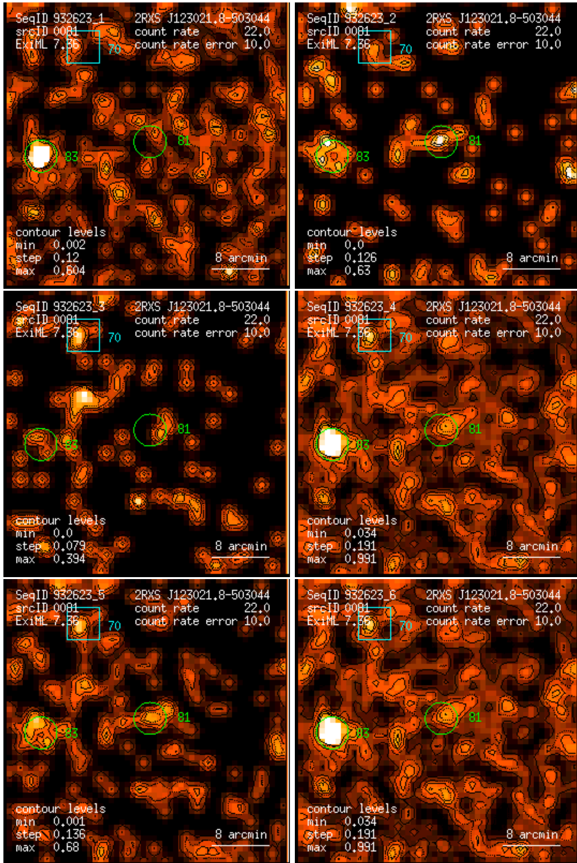
Figure 81: RASS 932623: detection 0081: band rate images, Gaussian filter: (1) PSPC channels 11 – 41, (2) 52 – 90, (3) 91 – 201, (4) 11 – 235, (5) 52 – 201, (6) 11 – 201. Broad band rates in counts/ks. Band rate contour levels in counts/ks/arcmin 2 .
