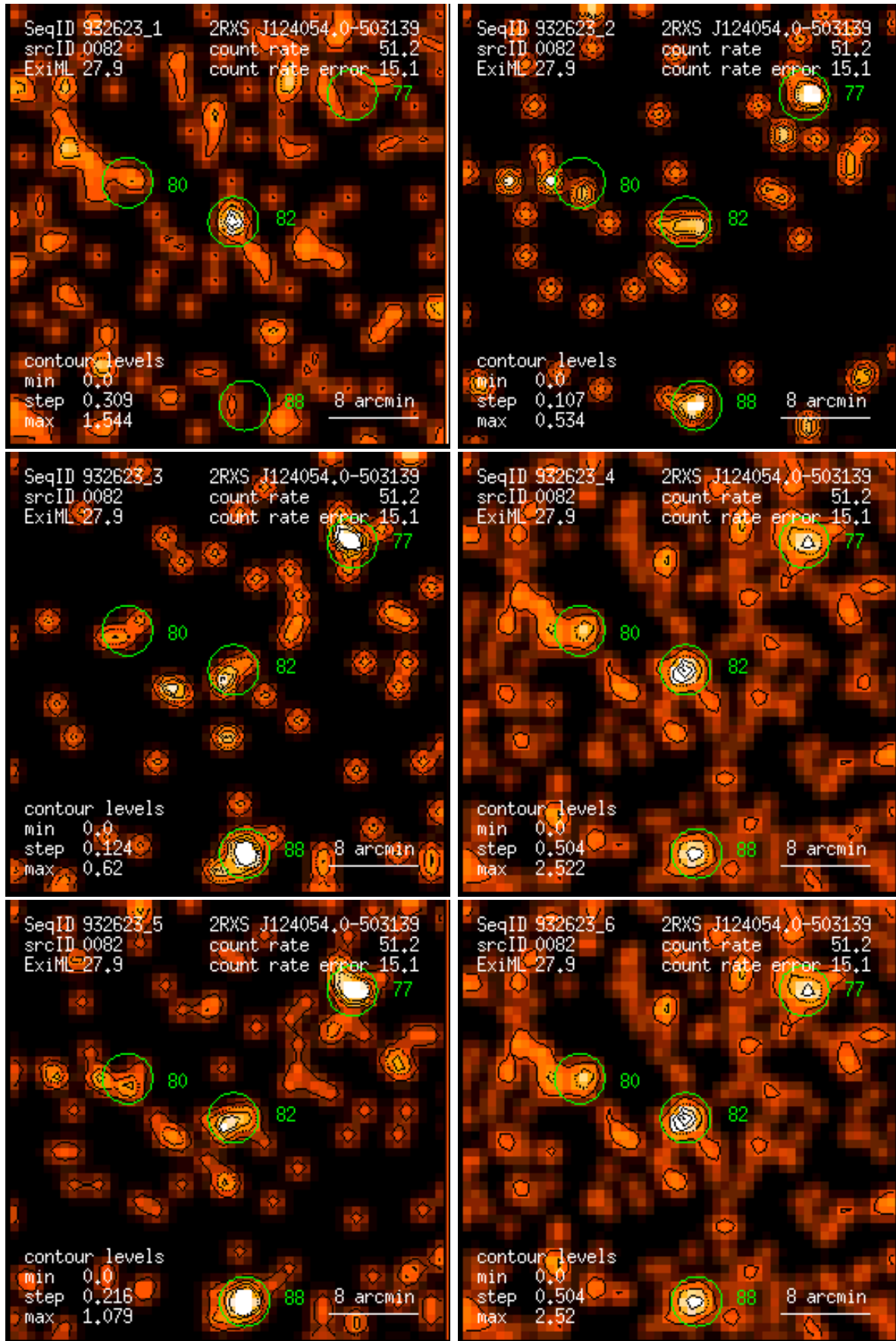
Figure 82: RASS 932623: detection 0082: band rate images, Gaussian filter: (1) PSPC channels 11 – 41, (2) 52 – 90, (3) 91 – 201, (4) 11 – 235, (5) 52 – 201, (6) 11 – 201. Broad band rates in counts/ks. Band rate contour levels in counts/ks/arcmin 2 .
