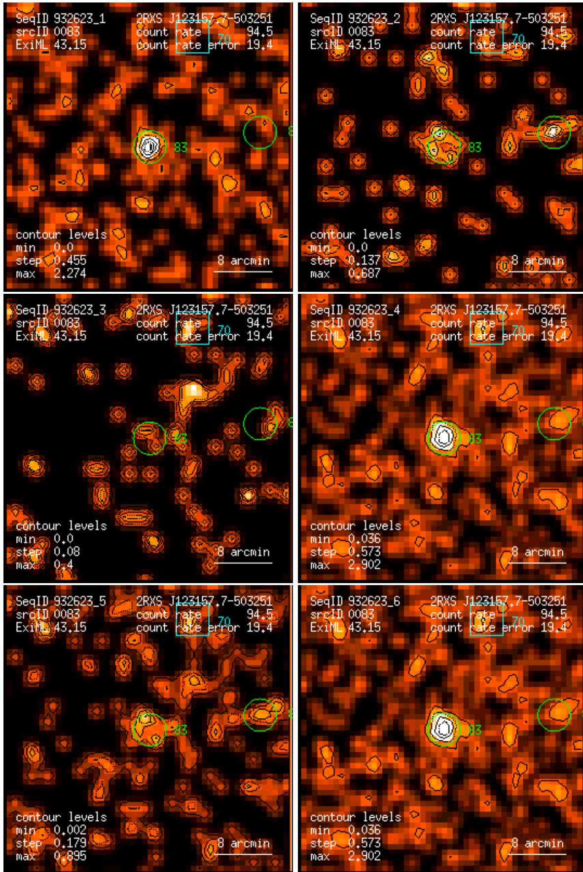
Figure 83: RASS 932623: detection 0083: band rate images, Gaussian filter: (1) PSPC channels 11 – 41, (2) 52 – 90, (3) 91 – 201, (4) 11 – 235, (5) 52 – 201, (6) 11 – 201. Broad band rates in counts/ks. Band rate contour levels in counts/ks/arcmin 2 .
