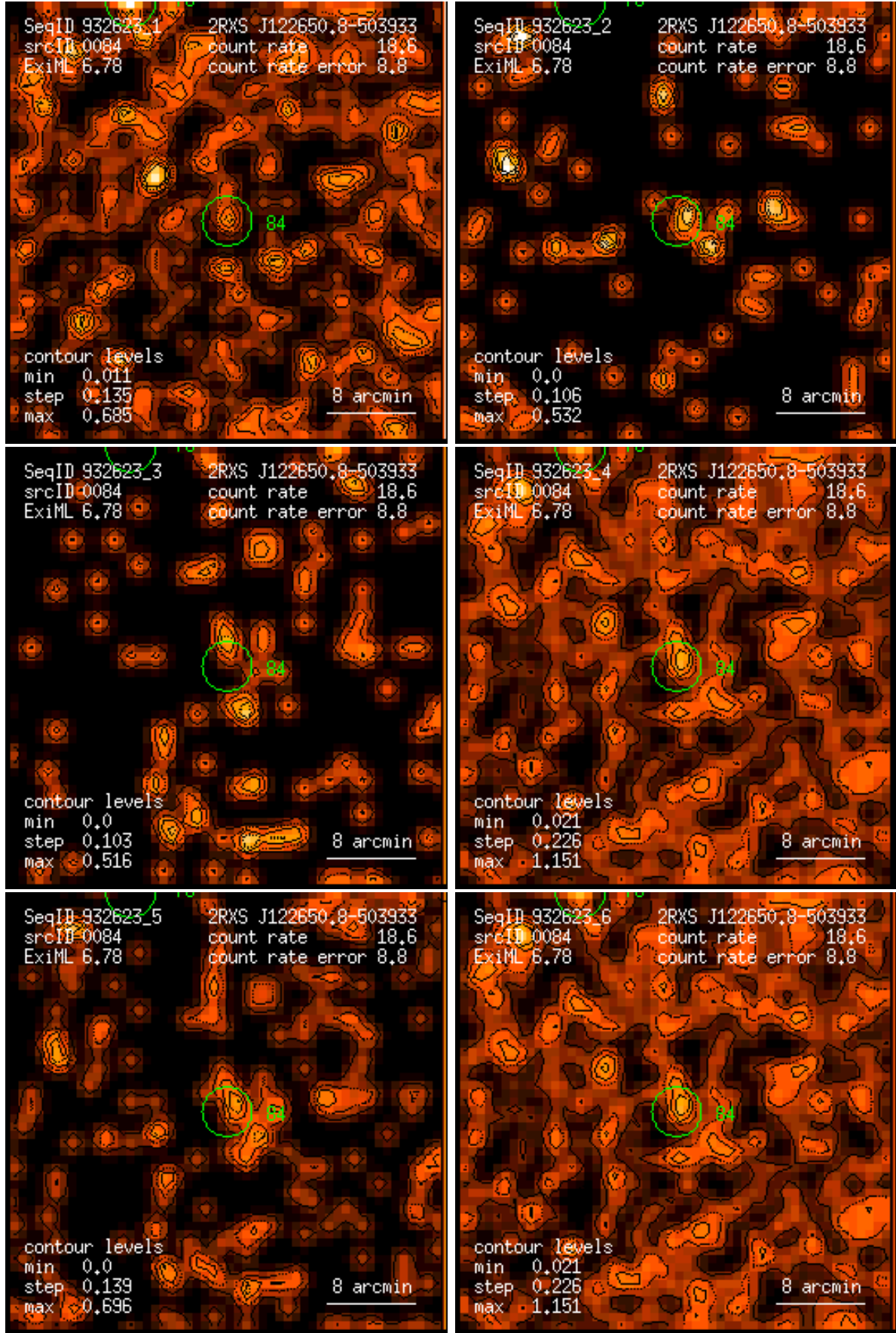
Figure 84: RASS 932623: detection 0084: band rate images, Gaussian filter: (1) PSPC channels 11 – 41, (2) 52 – 90, (3) 91 – 201, (4) 11 – 235, (5) 52 – 201, (6) 11 – 201. Broad band rates in counts/ks. Band rate contour levels in counts/ks/arcmin 2 .
