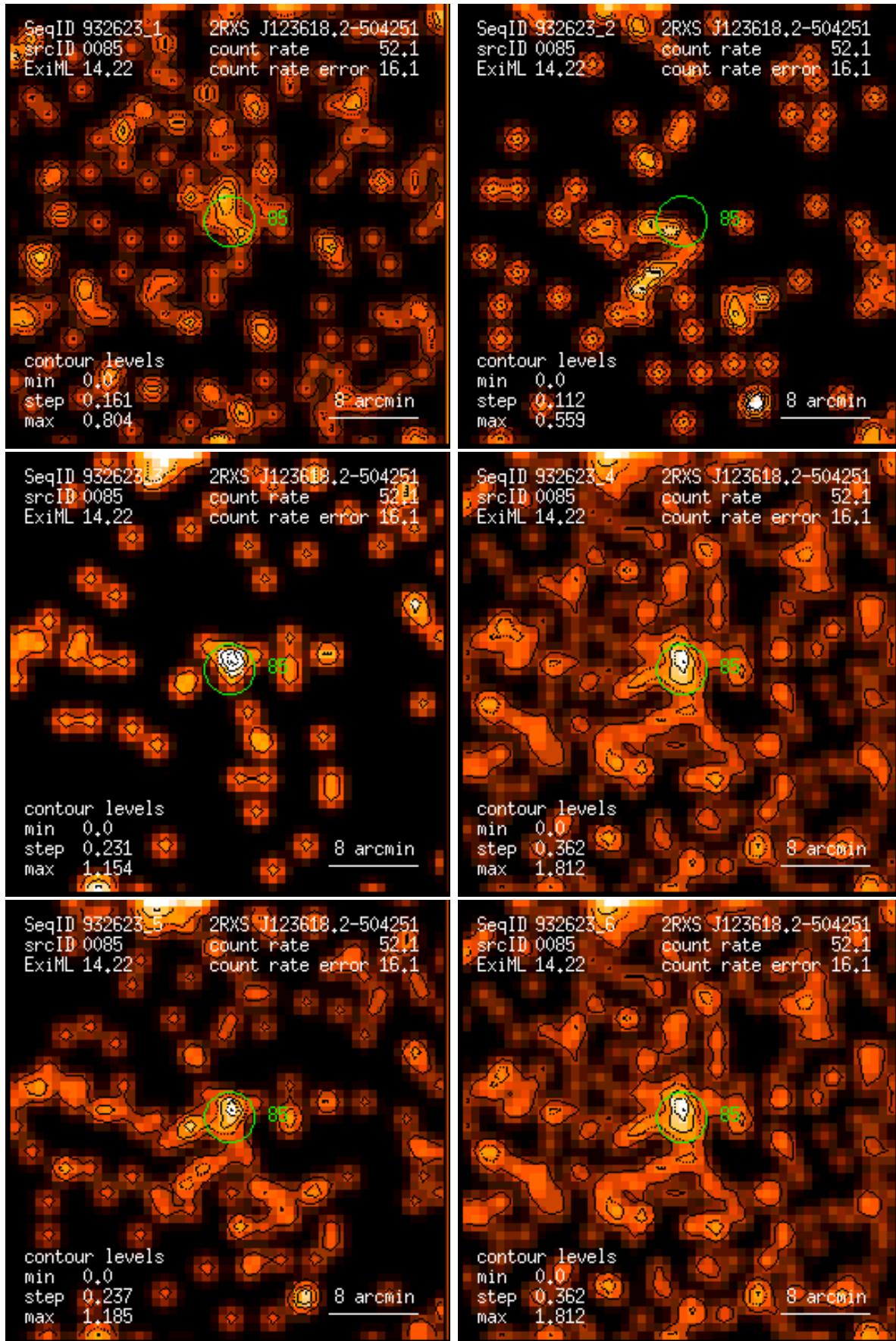
Figure 85: RASS 932623: detection 0085: band rate images, Gaussian filter: (1) PSPC channels 11 – 41, (2) 52 – 90, (3) 91 – 201, (4) 11 – 235, (5) 52 – 201, (6) 11 – 201. Broad band rates in counts/ks. Band rate contour levels in counts/ks/arcmin 2 .
