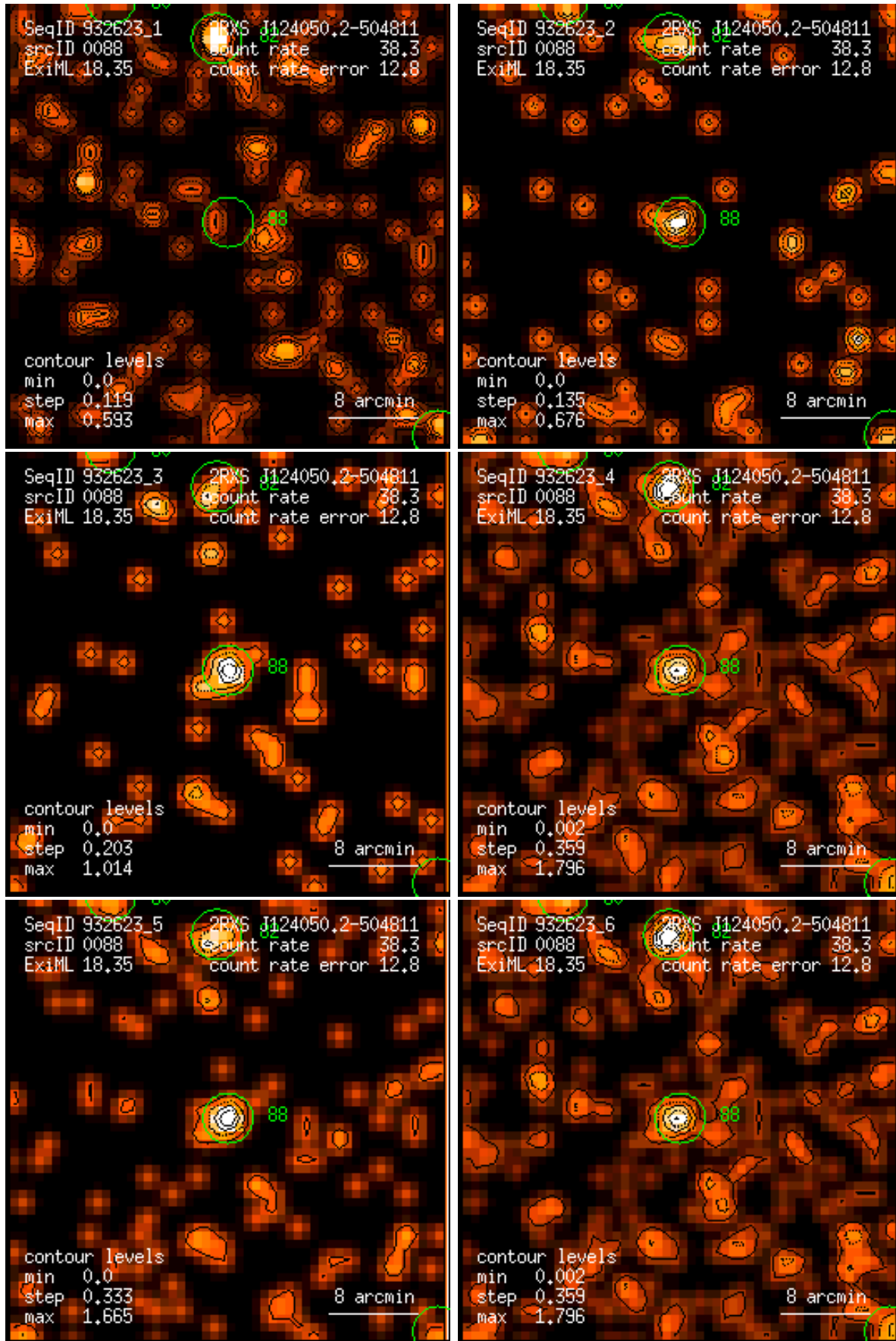
Figure 88: RASS 932623: detection 0088: band rate images, Gaussian filter: (1) PSPC channels 11 – 41, (2) 52 – 90, (3) 91 – 201, (4) 11 – 235, (5) 52 – 201, (6) 11 – 201. Broad band rates in counts/ks. Band rate contour levels in counts/ks/arcmin 2 .
