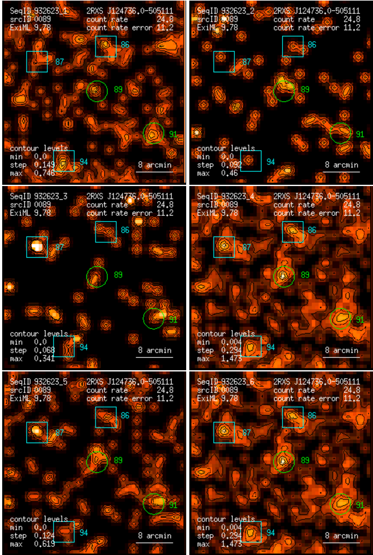
Figure 89: RASS 932623: detection 0089: band rate images, Gaussian filter: (1) PSPC channels 11 – 41, (2) 52 – 90, (3) 91 – 201, (4) 11 – 235, (5) 52 – 201, (6) 11 – 201. Broad band rates in counts/ks. Band rate contour levels in counts/ks/arcmin 2 .
