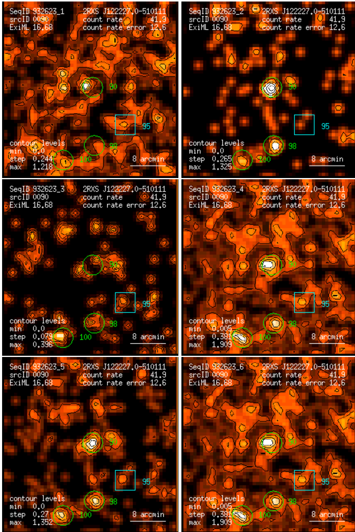
Figure 90: RASS 932623: detection 0090: band rate images, Gaussian filter: (1) PSPC channels 11 – 41, (2) 52 – 90, (3) 91 – 201, (4) 11 – 235, (5) 52 – 201, (6) 11 – 201. Broad band rates in counts/ks. Band rate contour levels in counts/ks/arcmin 2 .
