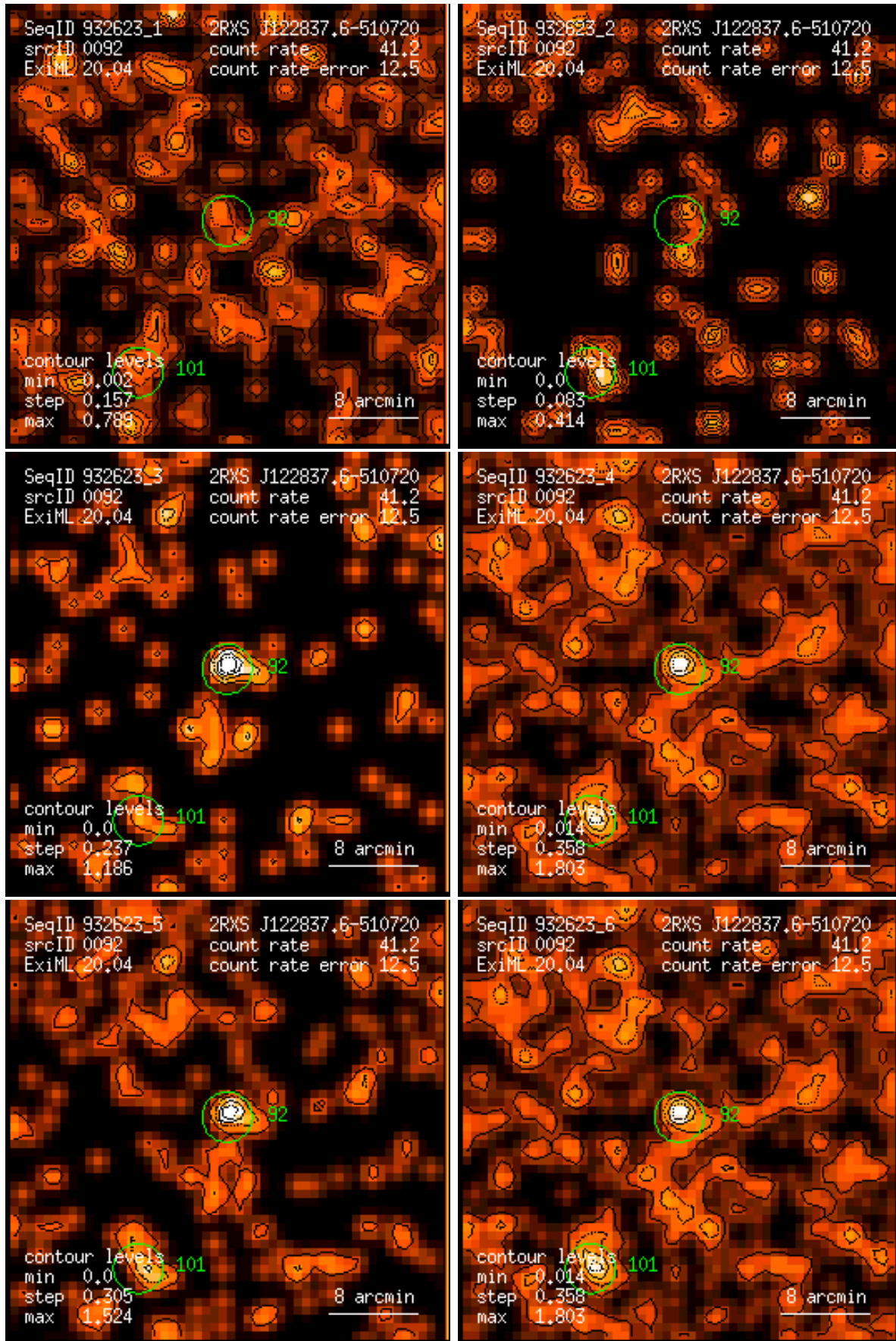
Figure 92: RASS 932623: detection 0092: band rate images, Gaussian filter: (1) PSPC channels 11 – 41, (2) 52 – 90, (3) 91 – 201, (4) 11 – 235, (5) 52 – 201, (6) 11 – 201. Broad band rates in counts/ks. Band rate contour levels in counts/ks/arcmin 2 .
