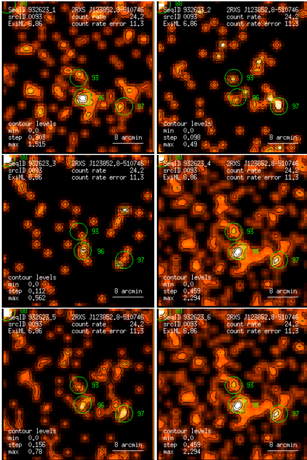
Figure 93: RASS 932623: detection 0093: band rate images, Gaussian filter: (1) PSPC channels 11 – 41, (2) 52 – 90, (3) 91 – 201, (4) 11 – 235, (5) 52 – 201, (6) 11 – 201. Broad band rates in counts/ks. Band rate contour levels in counts/ks/arcmin 2 .
