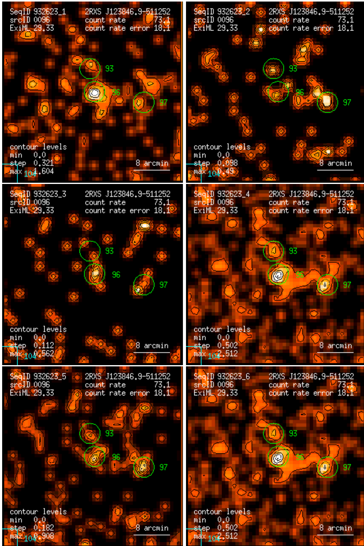
Figure 96: RASS 932623: detection 0096: band rate images, Gaussian filter: (1) PSPC channels 11 – 41, (2) 52 – 90, (3) 91 – 201, (4) 11 – 235, (5) 52 – 201, (6) 11 – 201. Broad band rates in counts/ks. Band rate contour levels in counts/ks/arcmin 2 .
