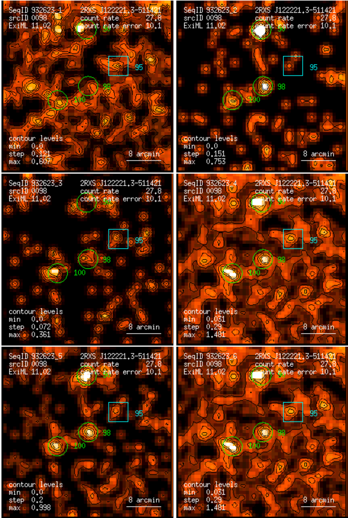
Figure 98: RASS 932623: detection 0098: band rate images, Gaussian filter: (1) PSPC channels 11 – 41, (2) 52 – 90, (3) 91 – 201, (4) 11 – 235, (5) 52 – 201, (6) 11 – 201. Broad band rates in counts/ks. Band rate contour levels in counts/ks/arcmin 2 .
