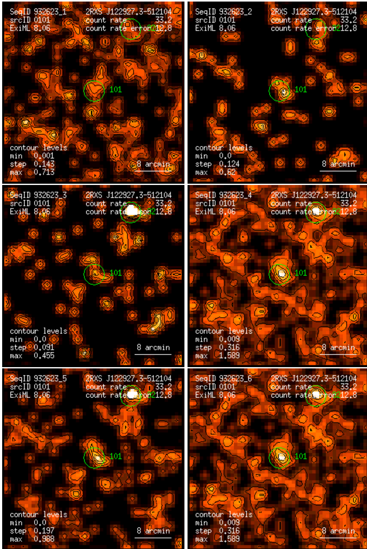
Figure 101: RASS 932623: detection 0101: band rate images, Gaussian filter: (1) PSPC channels 11 – 41, (2) 52 – 90, (3) 91 – 201, (4) 11 – 235, (5) 52 – 201, (6) 11 – 201. Broad band rates in counts/ks. Band rate contour levels in counts/ks/arcmin 2 .
