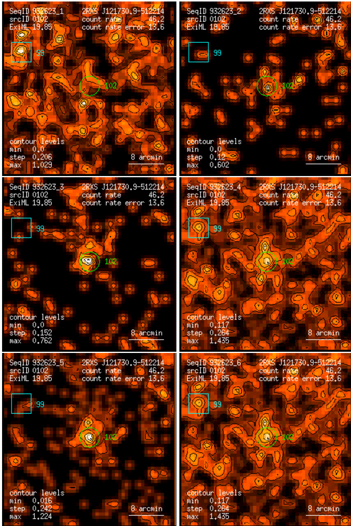
Figure 102: RASS 932623: detection 0102: band rate images, Gaussian filter: (1) PSPC channels 11 – 41, (2) 52 – 90, (3) 91 – 201, (4) 11 – 235, (5) 52 – 201, (6) 11 – 201. Broad band rates in counts/ks. Band rate contour levels in counts/ks/arcmin 2 .
