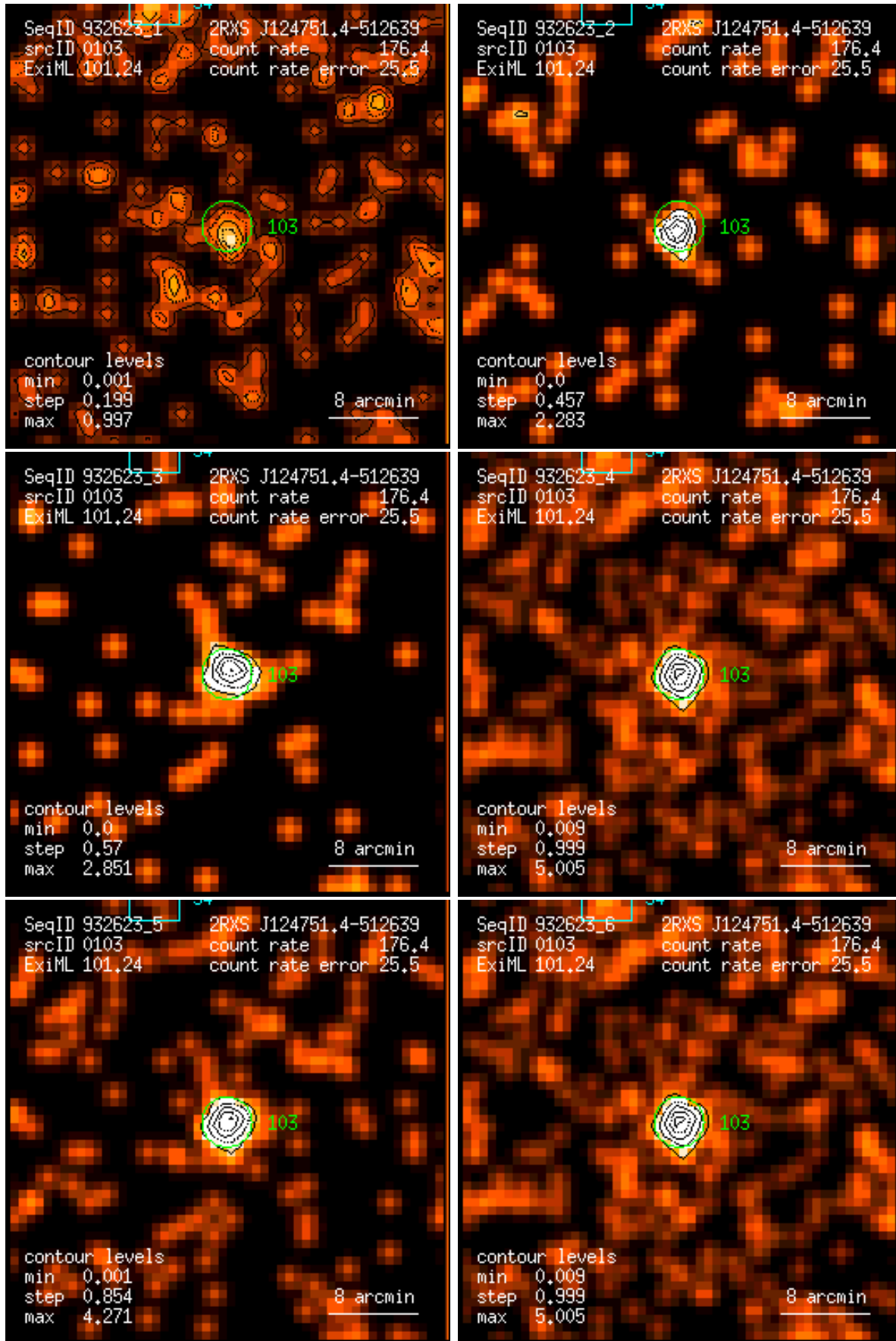
Figure 103: RASS 932623: detection 0103: band rate images, Gaussian filter: (1) PSPC channels 11 – 41, (2) 52 – 90, (3) 91 – 201, (4) 11 – 235, (5) 52 – 201, (6) 11 – 201. Broad band rates in counts/ks. Band rate contour levels in counts/ks/arcmin 2 .
