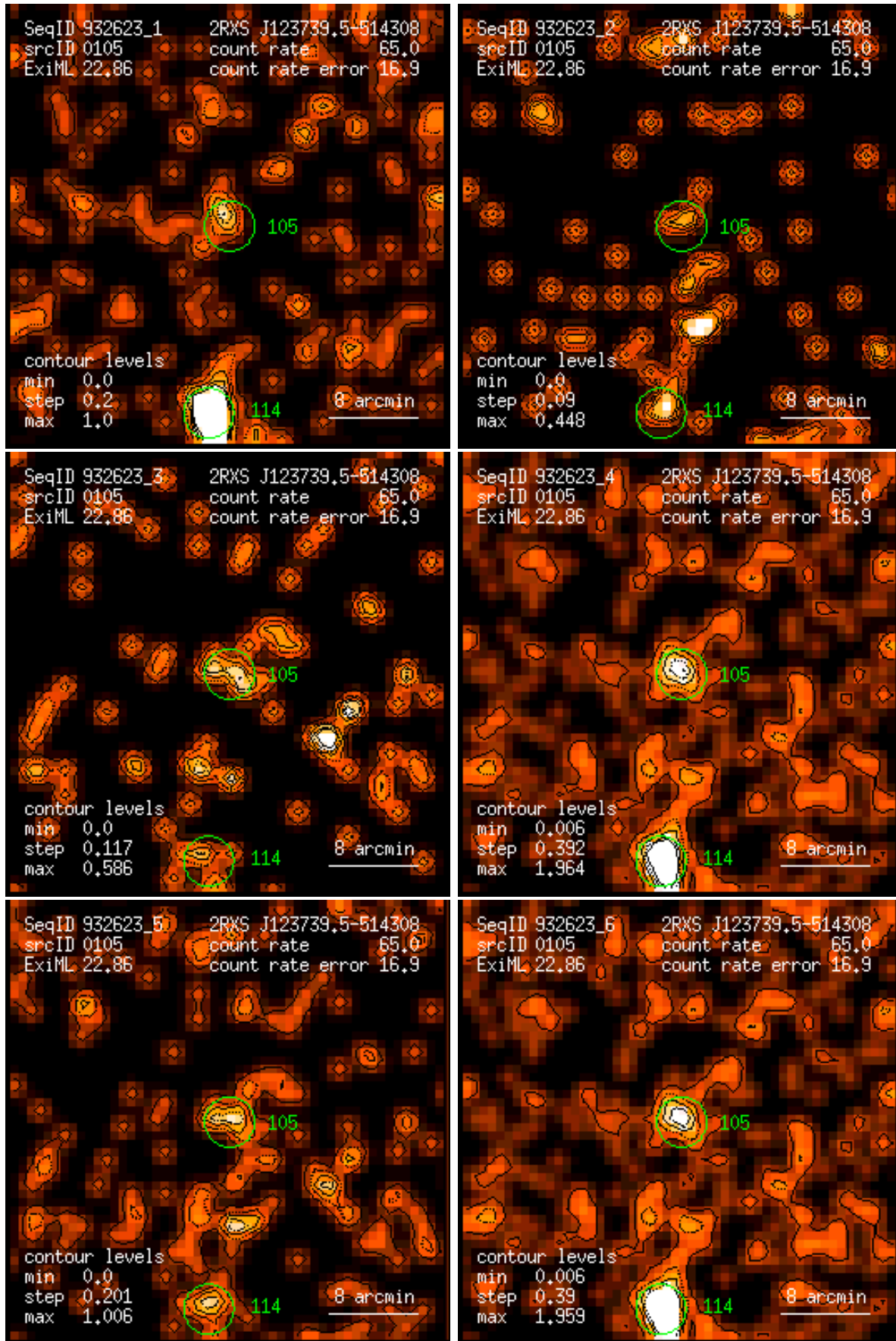
Figure 105: RASS 932623: detection 0105: band rate images, Gaussian filter: (1) PSPC channels 11 – 41, (2) 52 – 90, (3) 91 – 201, (4) 11 – 235, (5) 52 – 201, (6) 11 – 201. Broad band rates in counts/ks. Band rate contour levels in counts/ks/arcmin 2 .
