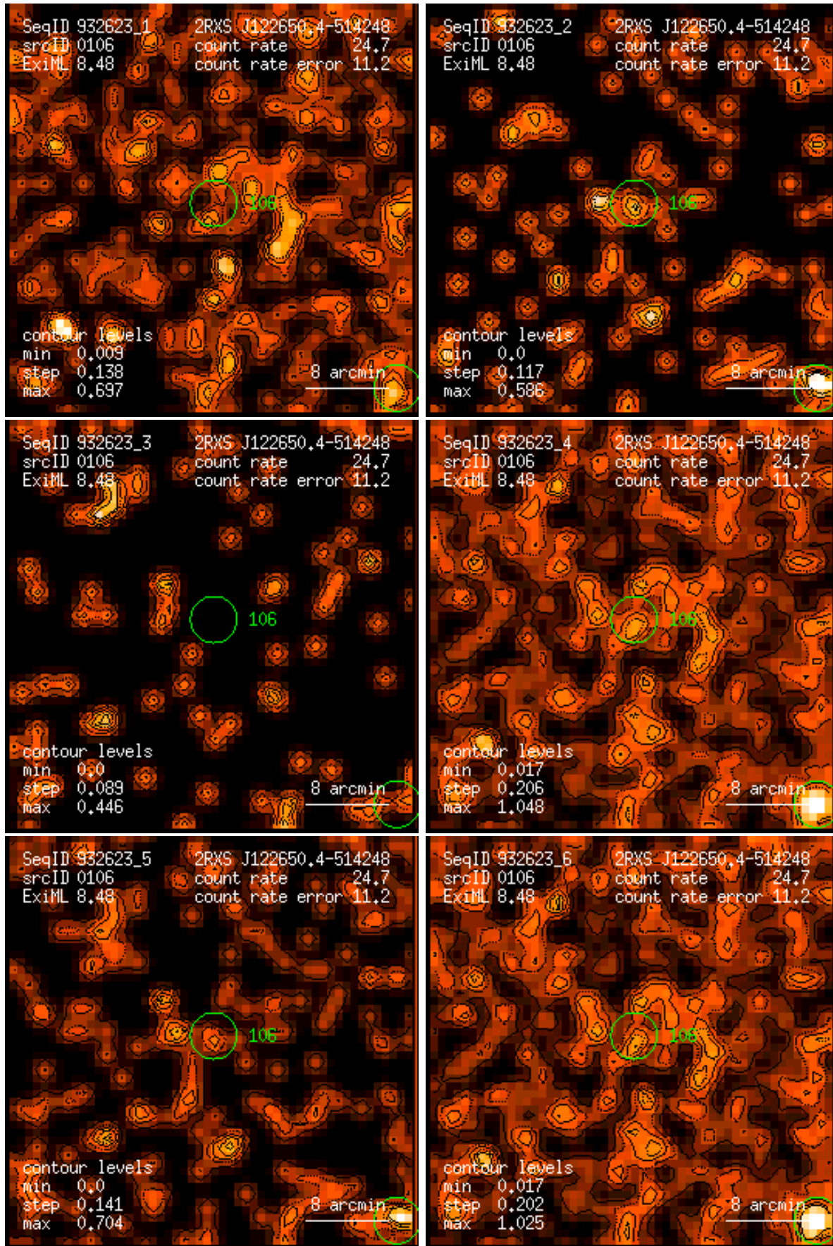
Figure 106: RASS 932623: detection 0106: band rate images, Gaussian filter: (1) PSPC channels 11 – 41, (2) 52 – 90, (3) 91 – 201, (4) 11 – 235, (5) 52 – 201, (6) 11 – 201. Broad band rates in counts/ks. Band rate contour levels in counts/ks/arcmin 2 .
