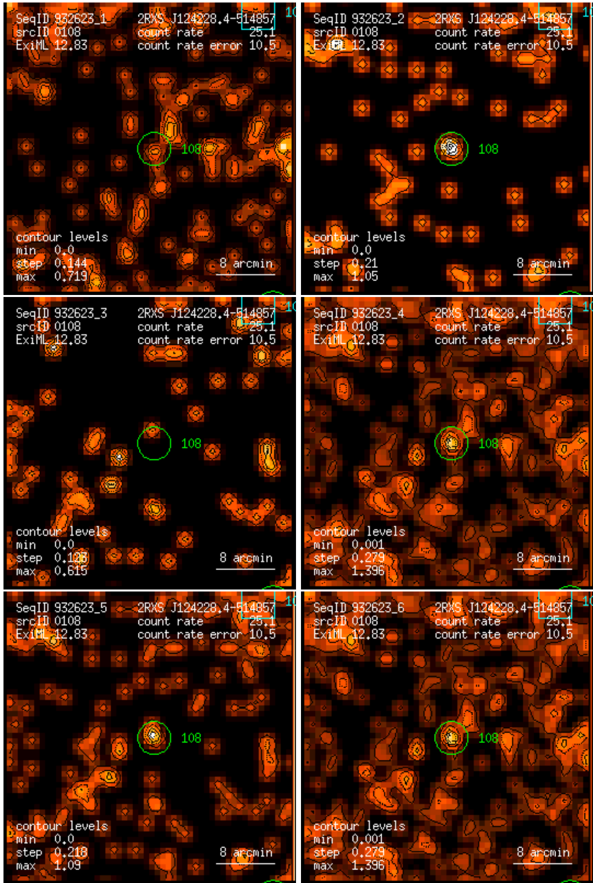
Figure 108: RASS 932623: detection 0108: band rate images, Gaussian filter: (1) PSPC channels 11 – 41, (2) 52 – 90, (3) 91 – 201, (4) 11 – 235, (5) 52 – 201, (6) 11 – 201. Broad band rates in counts/ks. Band rate contour levels in counts/ks/arcmin 2 .
