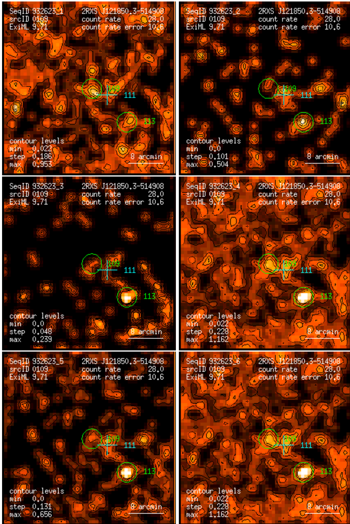
Figure 109: RASS 932623: detection 0109: band rate images, Gaussian filter: (1) PSPC channels 11 – 41, (2) 52 – 90, (3) 91 – 201, (4) 11 – 235, (5) 52 – 201, (6) 11 – 201. Broad band rates in counts/ks. Band rate contour levels in counts/ks/arcmin 2 .
