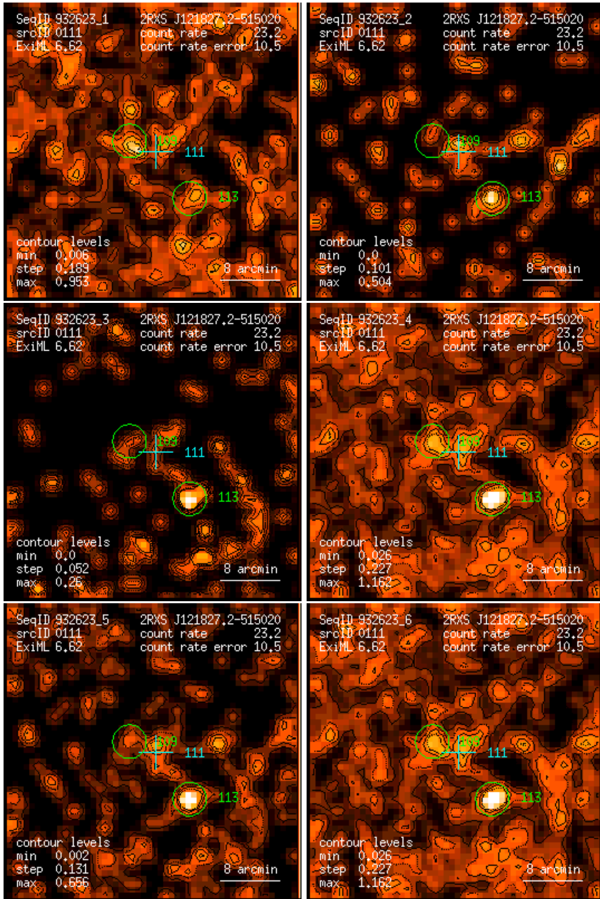
Figure 111: RASS 932623: detection 0111: band rate images, Gaussian filter: (1) PSPC channels 11 – 41, (2) 52 – 90, (3) 91 – 201, (4) 11 – 235, (5) 52 – 201, (6) 11 – 201. Broad band rates in counts/ks. Band rate contour levels in counts/ks/arcmin 2 .
