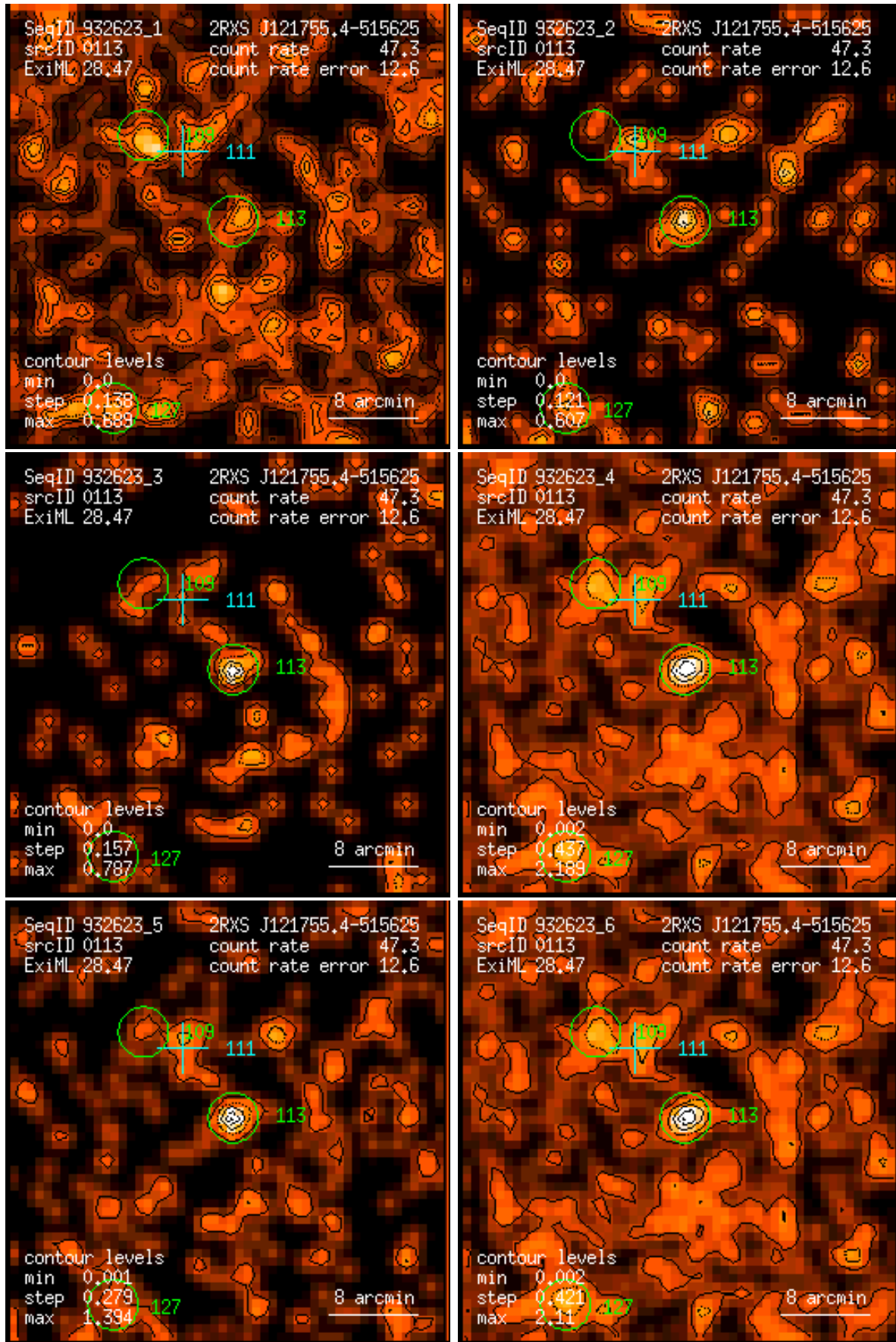
Figure 113: RASS 932623: detection 0113: band rate images, Gaussian filter: (1) PSPC channels 11 – 41, (2) 52 – 90, (3) 91 – 201, (4) 11 – 235, (5) 52 – 201, (6) 11 – 201. Broad band rates in counts/ks. Band rate contour levels in counts/ks/arcmin 2 .
