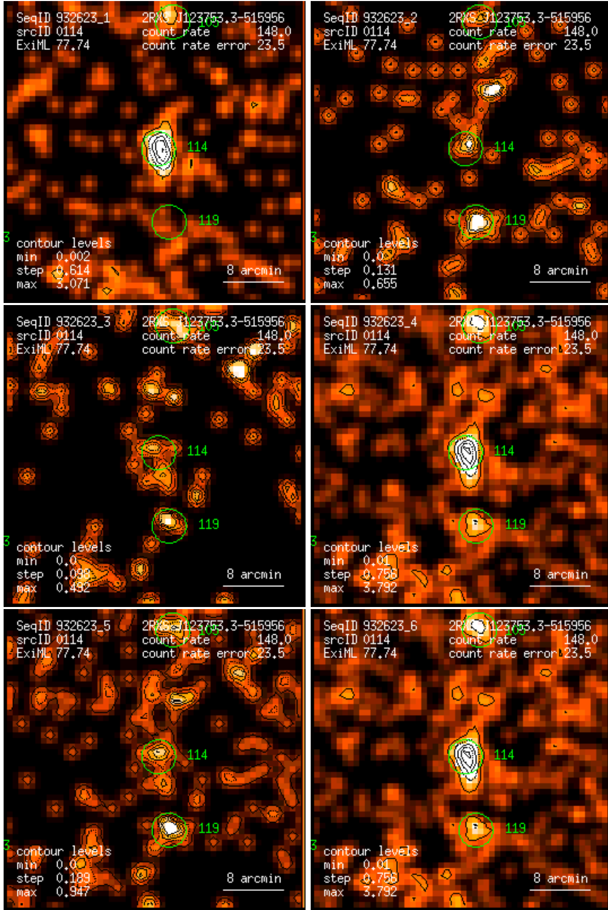
Figure 114: RASS 932623: detection 0114: band rate images, Gaussian filter: (1) PSPC channels 11 – 41, (2) 52 – 90, (3) 91 – 201, (4) 11 – 235, (5) 52 – 201, (6) 11 – 201. Broad band rates in counts/ks. Band rate contour levels in counts/ks/arcmin 2 .
