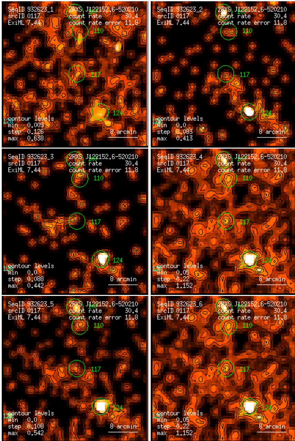
Figure 117: RASS 932623: detection 0117: band rate images, Gaussian filter: (1) PSPC channels 11 – 41, (2) 52 – 90, (3) 91 – 201, (4) 11 – 235, (5) 52 – 201, (6) 11 – 201. Broad band rates in counts/ks. Band rate contour levels in counts/ks/arcmin 2 .
