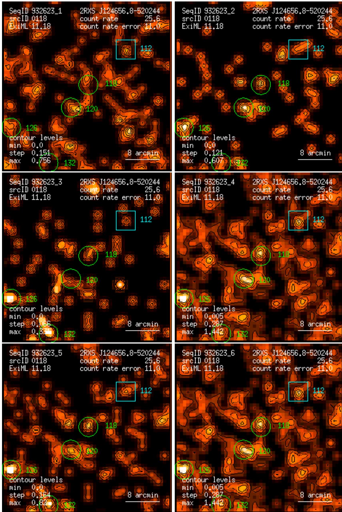
Figure 118: RASS 932623: detection 0118: band rate images, Gaussian filter: (1) PSPC channels 11 – 41, (2) 52 – 90, (3) 91 – 201, (4) 11 – 235, (5) 52 – 201, (6) 11 – 201. Broad band rates in counts/ks. Band rate contour levels in counts/ks/arcmin 2 .
