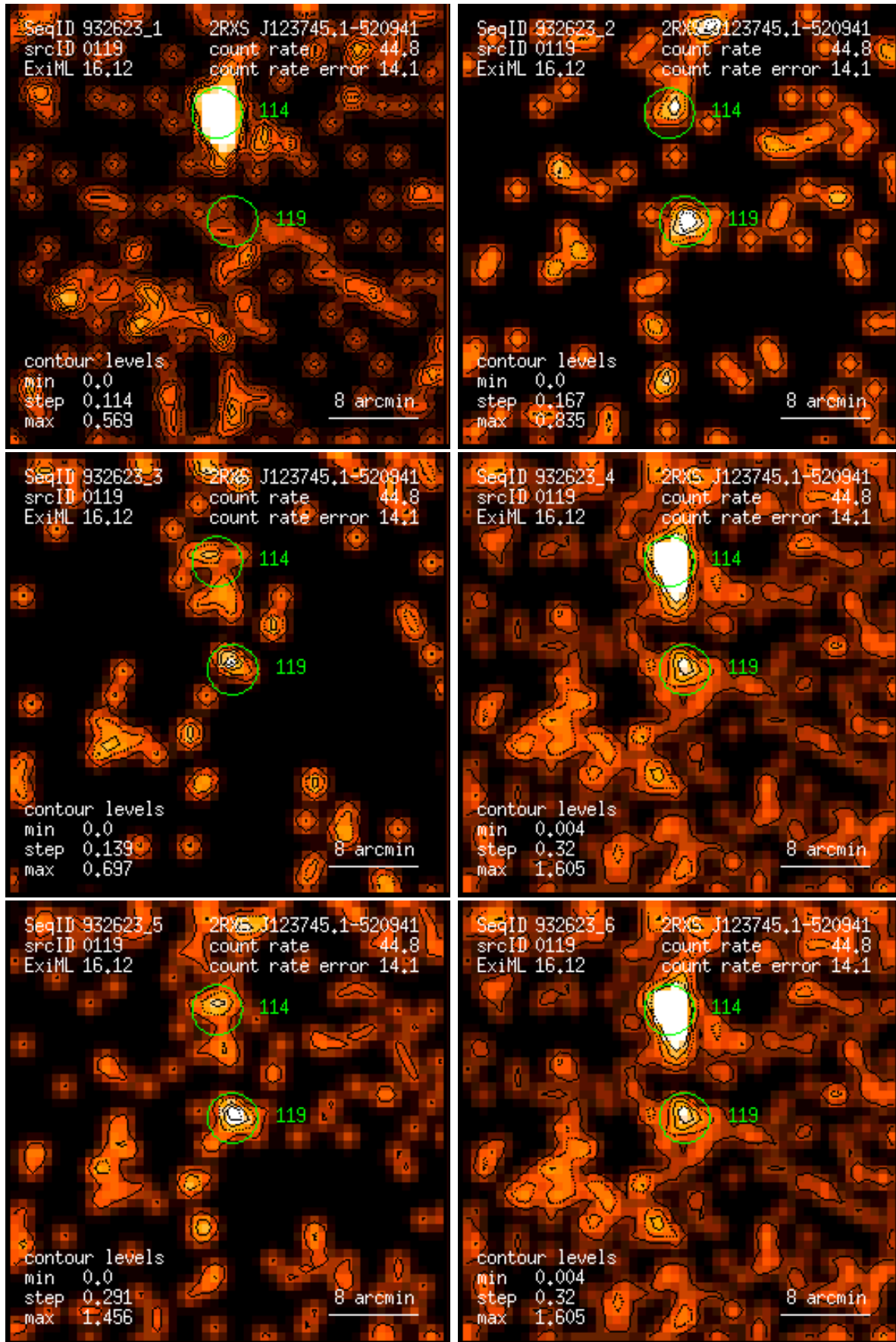
Figure 119: RASS 932623: detection 0119: band rate images, Gaussian filter: (1) PSPC channels 11 – 41, (2) 52 – 90, (3) 91 – 201, (4) 11 – 235, (5) 52 – 201, (6) 11 – 201. Broad band rates in counts/ks. Band rate contour levels in counts/ks/arcmin 2 .
