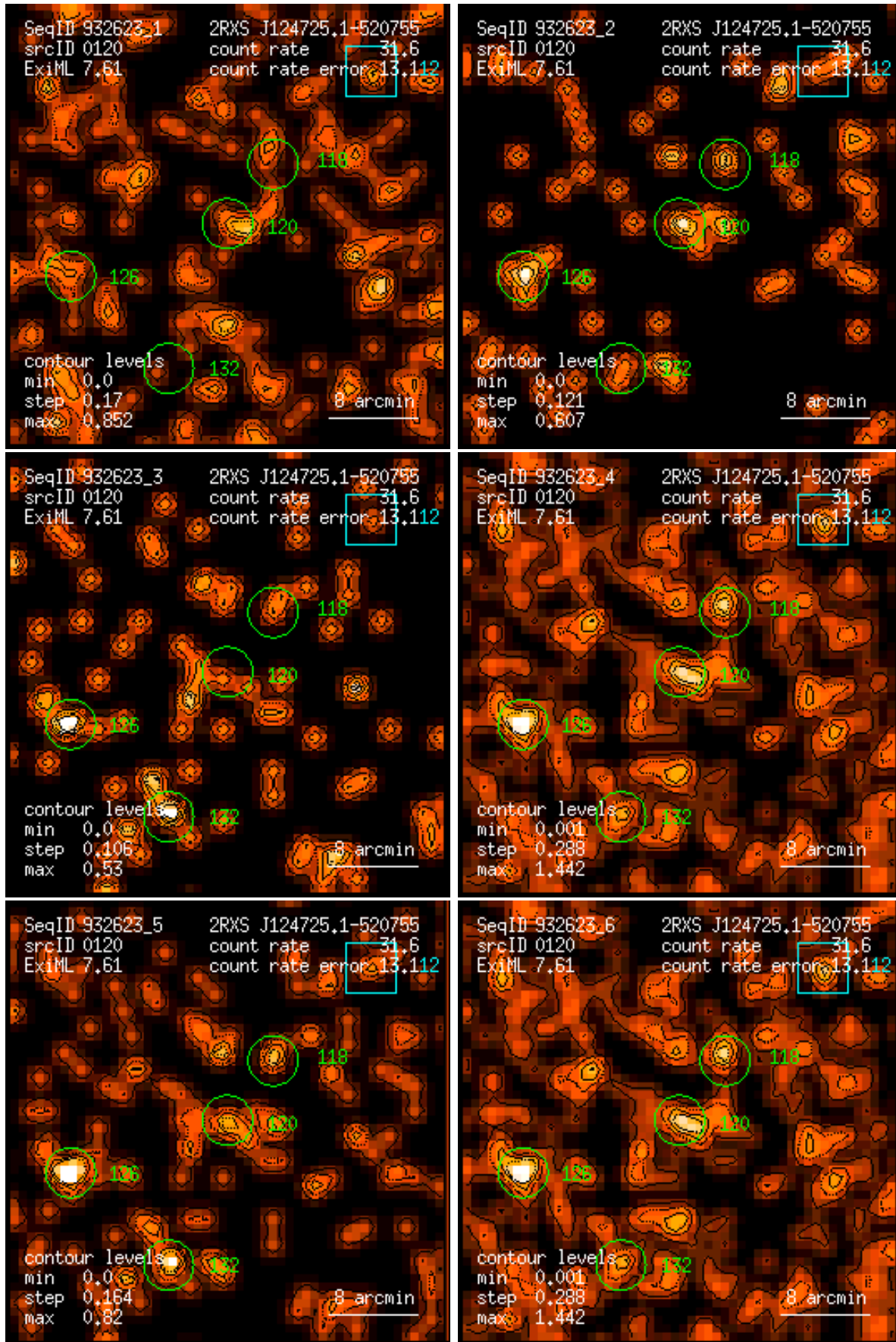
Figure 120: RASS 932623: detection 0120: band rate images, Gaussian filter: (1) PSPC channels 11 – 41, (2) 52 – 90, (3) 91 – 201, (4) 11 – 235, (5) 52 – 201, (6) 11 – 201. Broad band rates in counts/ks. Band rate contour levels in counts/ks/arcmin 2 .
