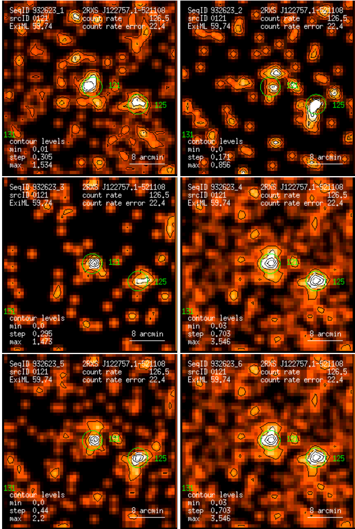
Figure 121: RASS 932623: detection 0121: band rate images, Gaussian filter: (1) PSPC channels 11 – 41, (2) 52 – 90, (3) 91 – 201, (4) 11 – 235, (5) 52 – 201, (6) 11 – 201. Broad band rates in counts/ks. Band rate contour levels in counts/ks/arcmin 2 .
