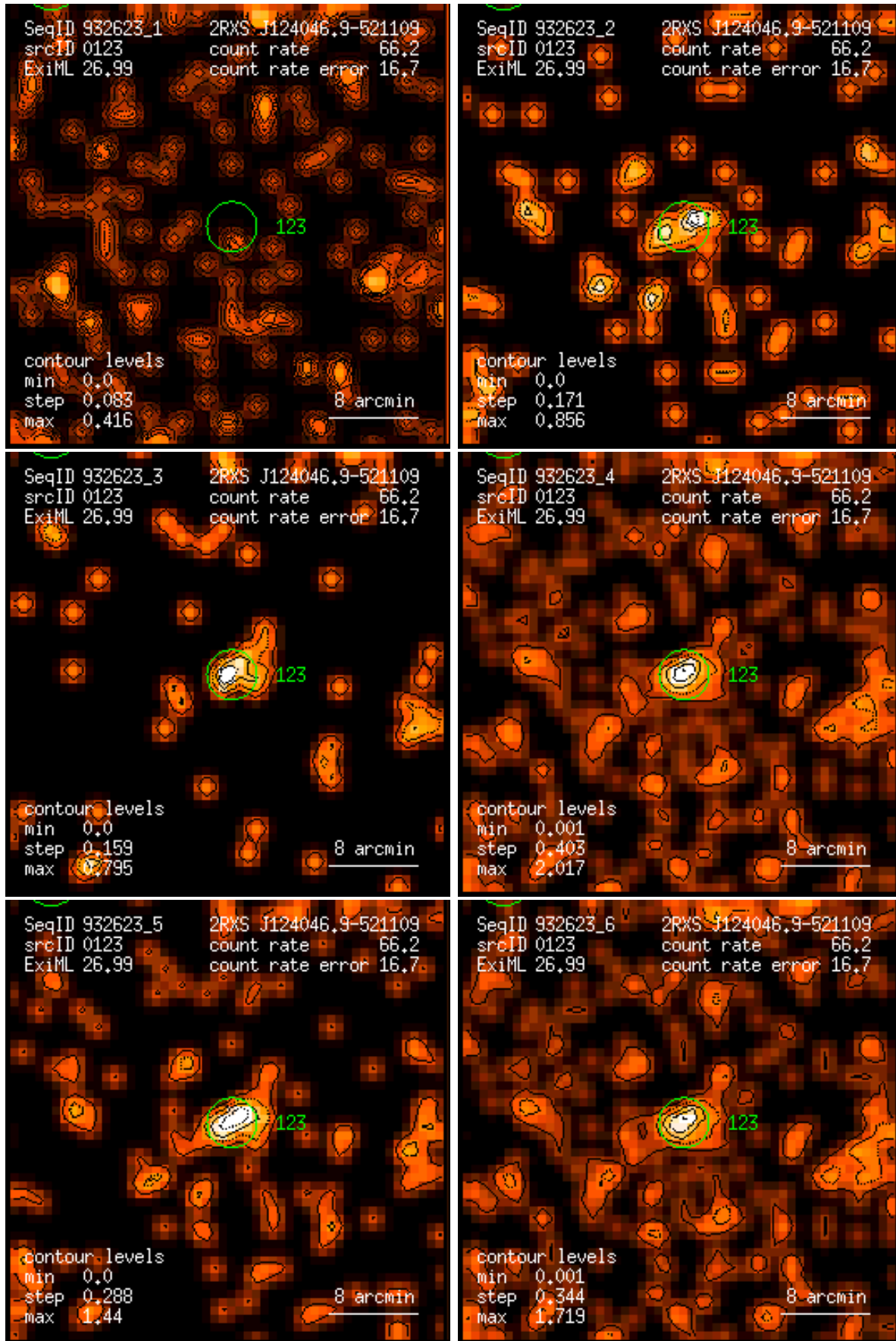
Figure 123: RASS 932623: detection 0123: band rate images, Gaussian filter: (1) PSPC channels 11 – 41, (2) 52 – 90, (3) 91 – 201, (4) 11 – 235, (5) 52 – 201, (6) 11 – 201. Broad band rates in counts/ks. Band rate contour levels in counts/ks/arcmin 2 .
