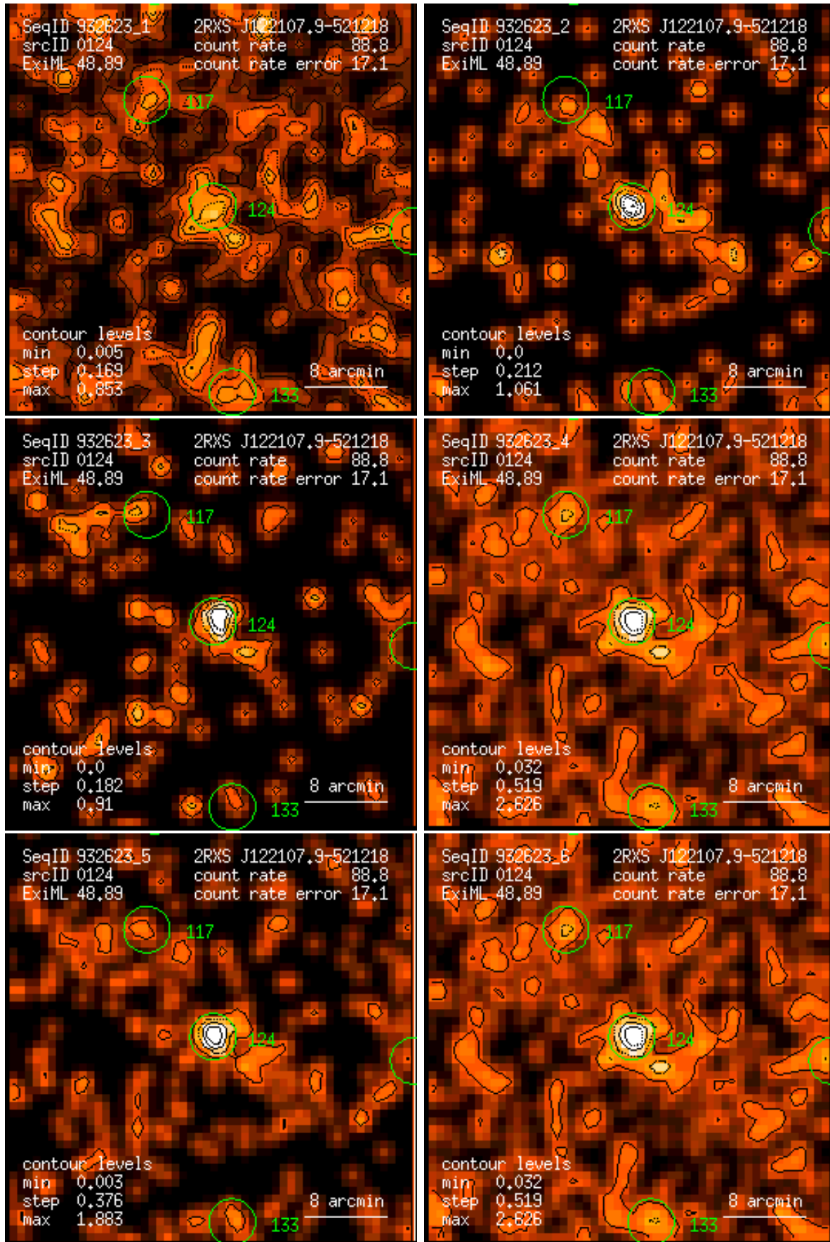
Figure 124: RASS 932623: detection 0124: band rate images, Gaussian filter: (1) PSPC channels 11 – 41, (2) 52 – 90, (3) 91 – 201, (4) 11 – 235, (5) 52 – 201, (6) 11 – 201. Broad band rates in counts/ks. Band rate contour levels in counts/ks/arcmin 2 .
