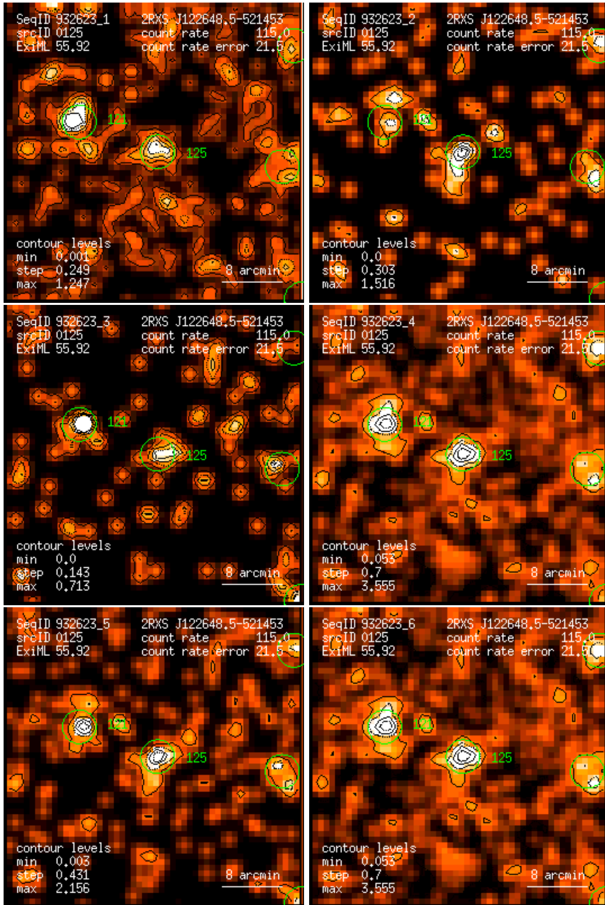
Figure 125: RASS 932623: detection 0125: band rate images, Gaussian filter: (1) PSPC channels 11 – 41, (2) 52 – 90, (3) 91 – 201, (4) 11 – 235, (5) 52 – 201, (6) 11 – 201. Broad band rates in counts/ks. Band rate contour levels in counts/ks/arcmin 2 .
