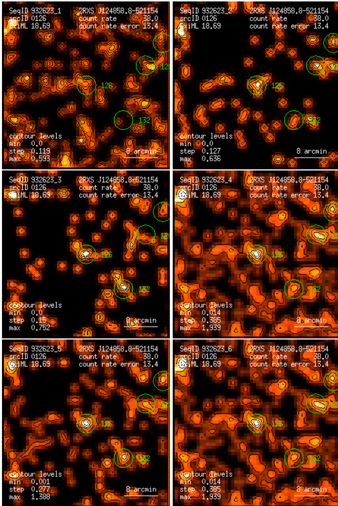
Figure 126: RASS 932623: detection 0126: band rate images, Gaussian filter: (1) PSPC channels 11 – 41, (2) 52 – 90, (3) 91 – 201, (4) 11 – 235, (5) 52 – 201, (6) 11 – 201. Broad band rates in counts/ks. Band rate contour levels in counts/ks/arcmin 2 .
