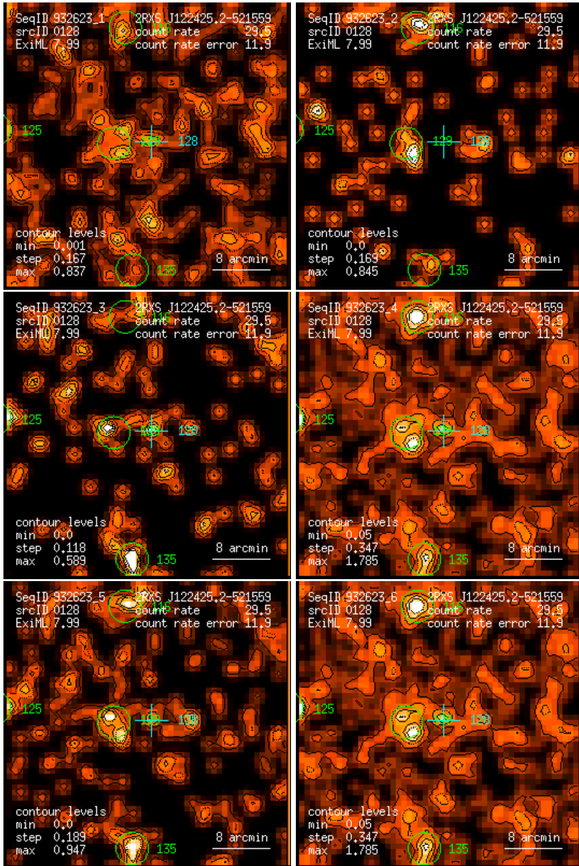
Figure 128: RASS 932623: detection 0128: band rate images, Gaussian filter: (1) PSPC channels 11 – 41, (2) 52 – 90, (3) 91 – 201, (4) 11 – 235, (5) 52 – 201, (6) 11 – 201. Broad band rates in counts/ks. Band rate contour levels in counts/ks/arcmin 2 .
