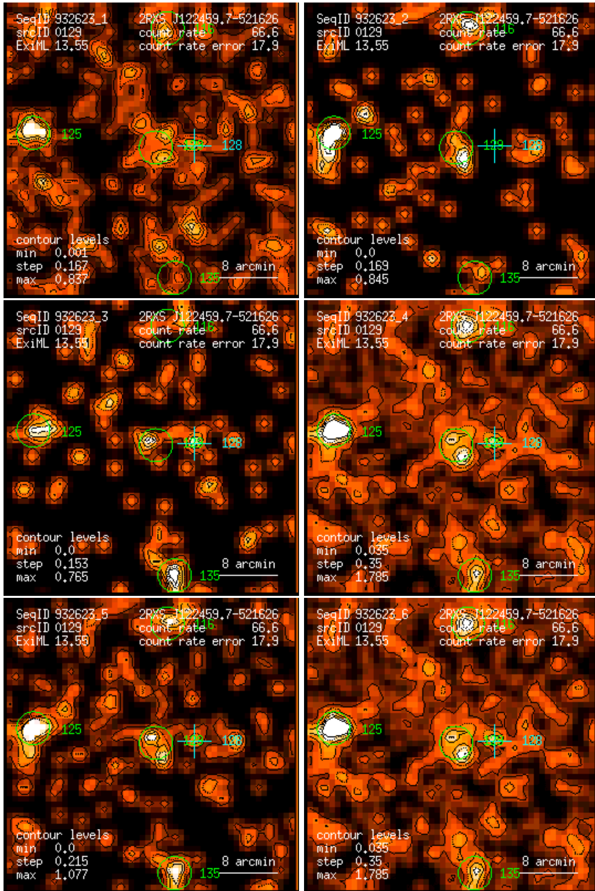
Figure 129: RASS 932623: detection 0129: band rate images, Gaussian filter: (1) PSPC channels 11 – 41, (2) 52 – 90, (3) 91 – 201, (4) 11 – 235, (5) 52 – 201, (6) 11 – 201. Broad band rates in counts/ks. Band rate contour levels in counts/ks/arcmin 2 .
