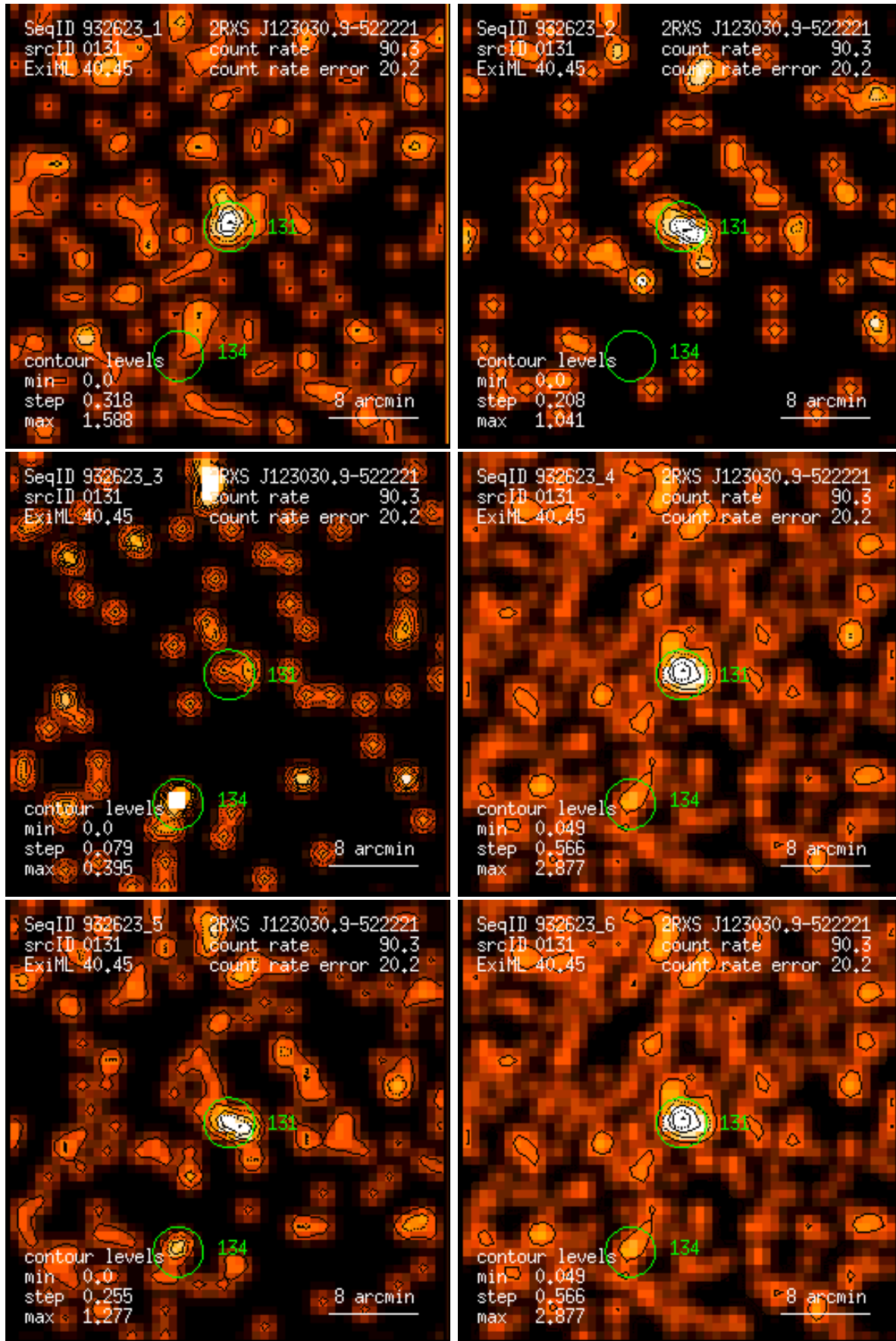
Figure 131: RASS 932623: detection 0131: band rate images, Gaussian filter: (1) PSPC channels 11 – 41, (2) 52 – 90, (3) 91 – 201, (4) 11 – 235, (5) 52 – 201, (6) 11 – 201. Broad band rates in counts/ks. Band rate contour levels in counts/ks/arcmin 2 .
