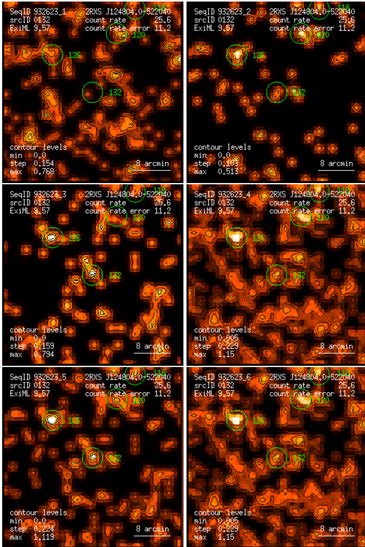
Figure 132: RASS 932623: detection 0132: band rate images, Gaussian filter: (1) PSPC channels 11 – 41, (2) 52 – 90, (3) 91 – 201, (4) 11 – 235, (5) 52 – 201, (6) 11 – 201. Broad band rates in counts/ks. Band rate contour levels in counts/ks/arcmin 2 .
