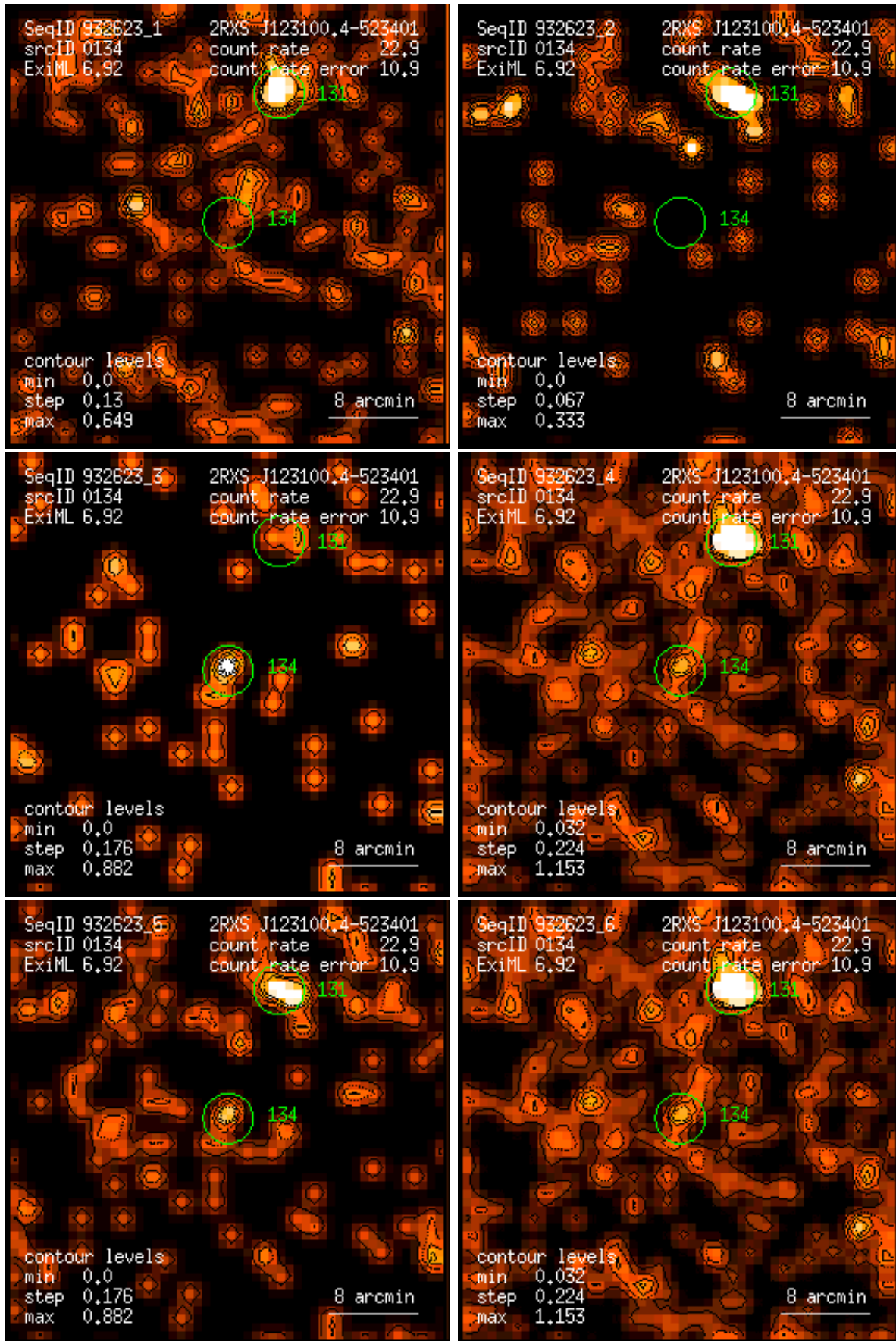
Figure 134: RASS 932623: detection 0134: band rate images, Gaussian filter: (1) PSPC channels 11 – 41, (2) 52 – 90, (3) 91 – 201, (4) 11 – 235, (5) 52 – 201, (6) 11 – 201. Broad band rates in counts/ks. Band rate contour levels in counts/ks/arcmin 2 .
