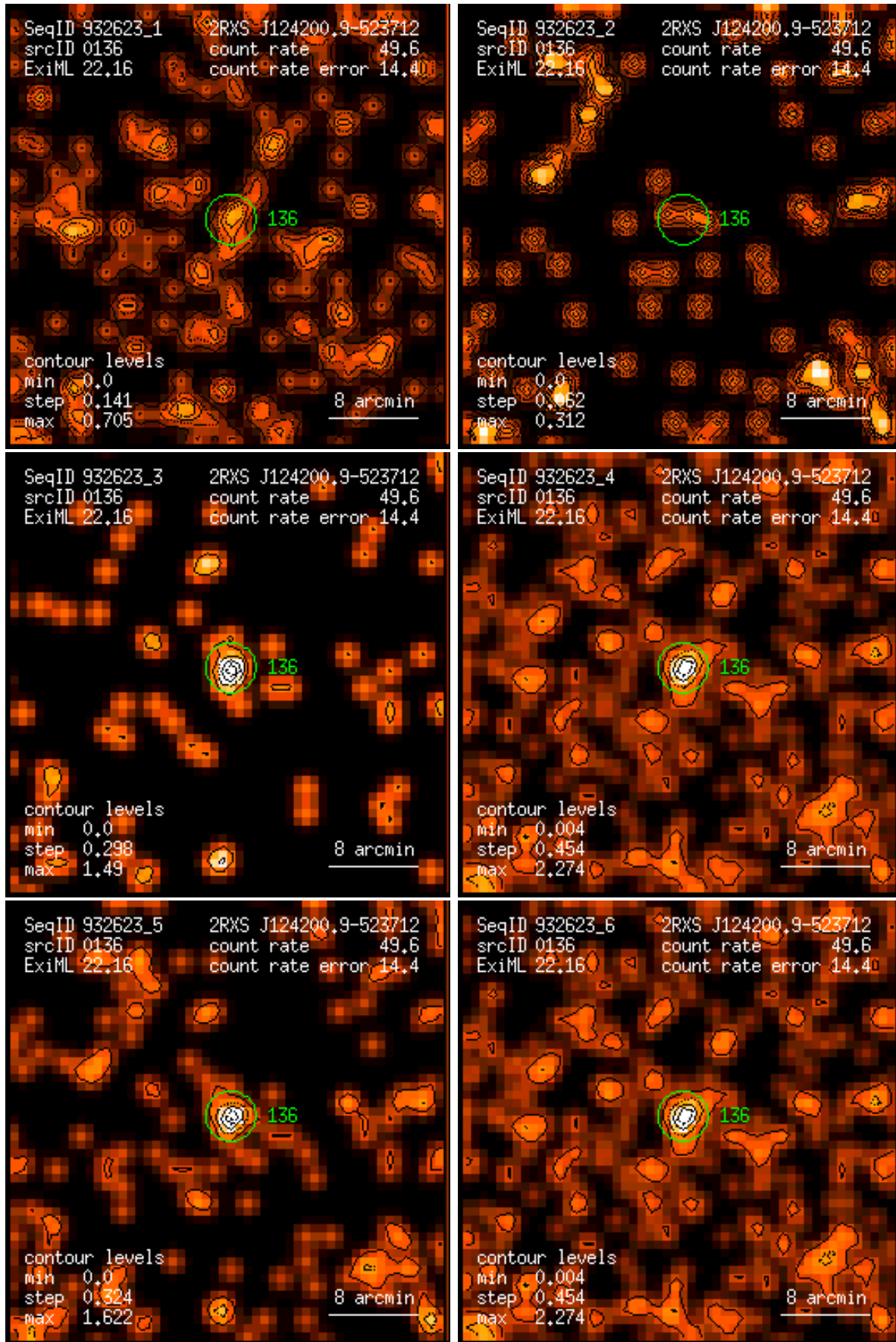
Figure 136: RASS 932623: detection 0136: band rate images, Gaussian filter: (1) PSPC channels 11 – 41, (2) 52 – 90, (3) 91 – 201, (4) 11 – 235, (5) 52 – 201, (6) 11 – 201. Broad band rates in counts/ks. Band rate contour levels in counts/ks/arcmin 2 .
