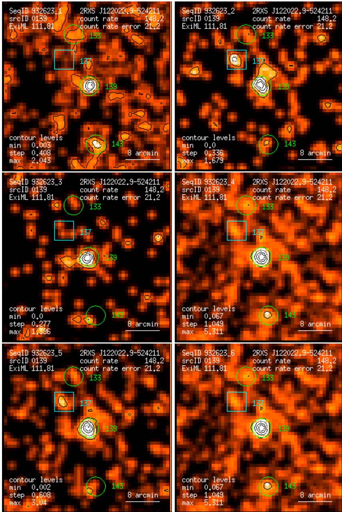
Figure 139: RASS 932623: detection 0139: band rate images, Gaussian filter: (1) PSPC channels 11 – 41, (2) 52 – 90, (3) 91 – 201, (4) 11 – 235, (5) 52 – 201, (6) 11 – 201. Broad band rates in counts/ks. Band rate contour levels in counts/ks/arcmin 2 .
