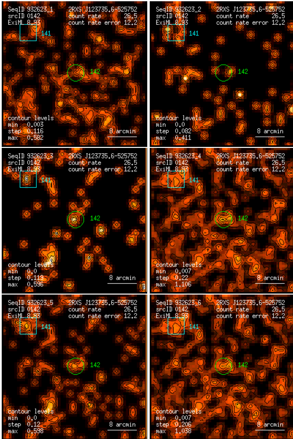
Figure 142: RASS 932623: detection 0142: band rate images, Gaussian filter: (1) PSPC channels 11 – 41, (2) 52 – 90, (3) 91 – 201, (4) 11 – 235, (5) 52 – 201, (6) 11 – 201. Broad band rates in counts/ks. Band rate contour levels in counts/ks/arcmin 2 .
