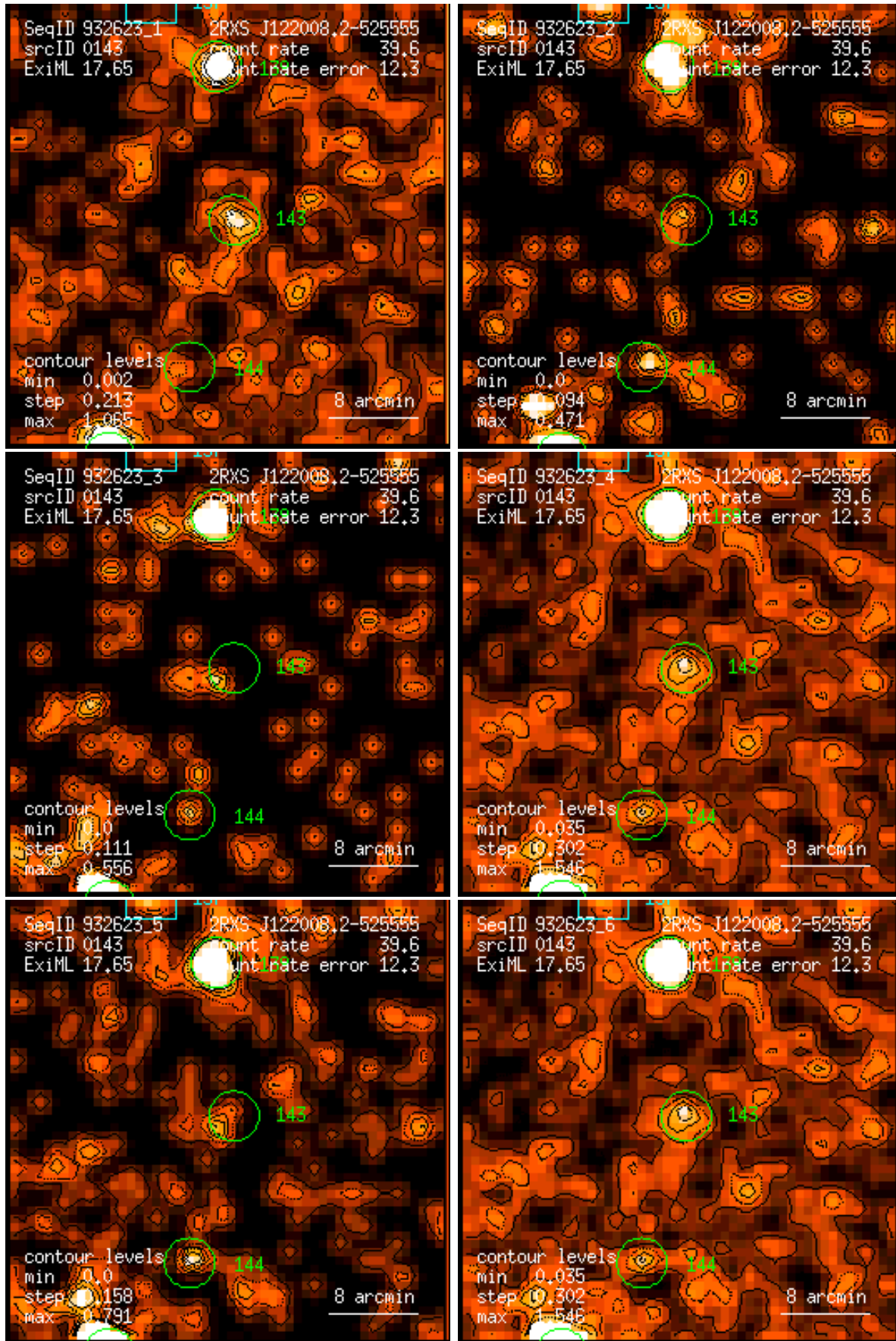
Figure 143: RASS 932623: detection 0143: band rate images, Gaussian filter: (1) PSPC channels 11 – 41, (2) 52 – 90, (3) 91 – 201, (4) 11 – 235, (5) 52 – 201, (6) 11 – 201. Broad band rates in counts/ks. Band rate contour levels in counts/ks/arcmin 2 .
