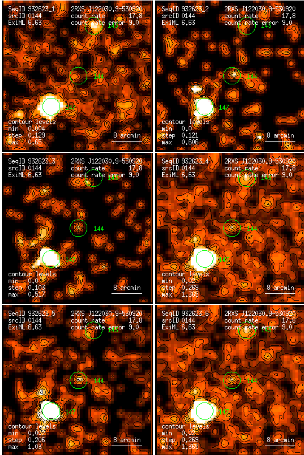
Figure 144: RASS 932623: detection 0144: band rate images, Gaussian filter: (1) PSPC channels 11 – 41, (2) 52 – 90, (3) 91 – 201, (4) 11 – 235, (5) 52 – 201, (6) 11 – 201. Broad band rates in counts/ks. Band rate contour levels in counts/ks/arcmin 2 .
