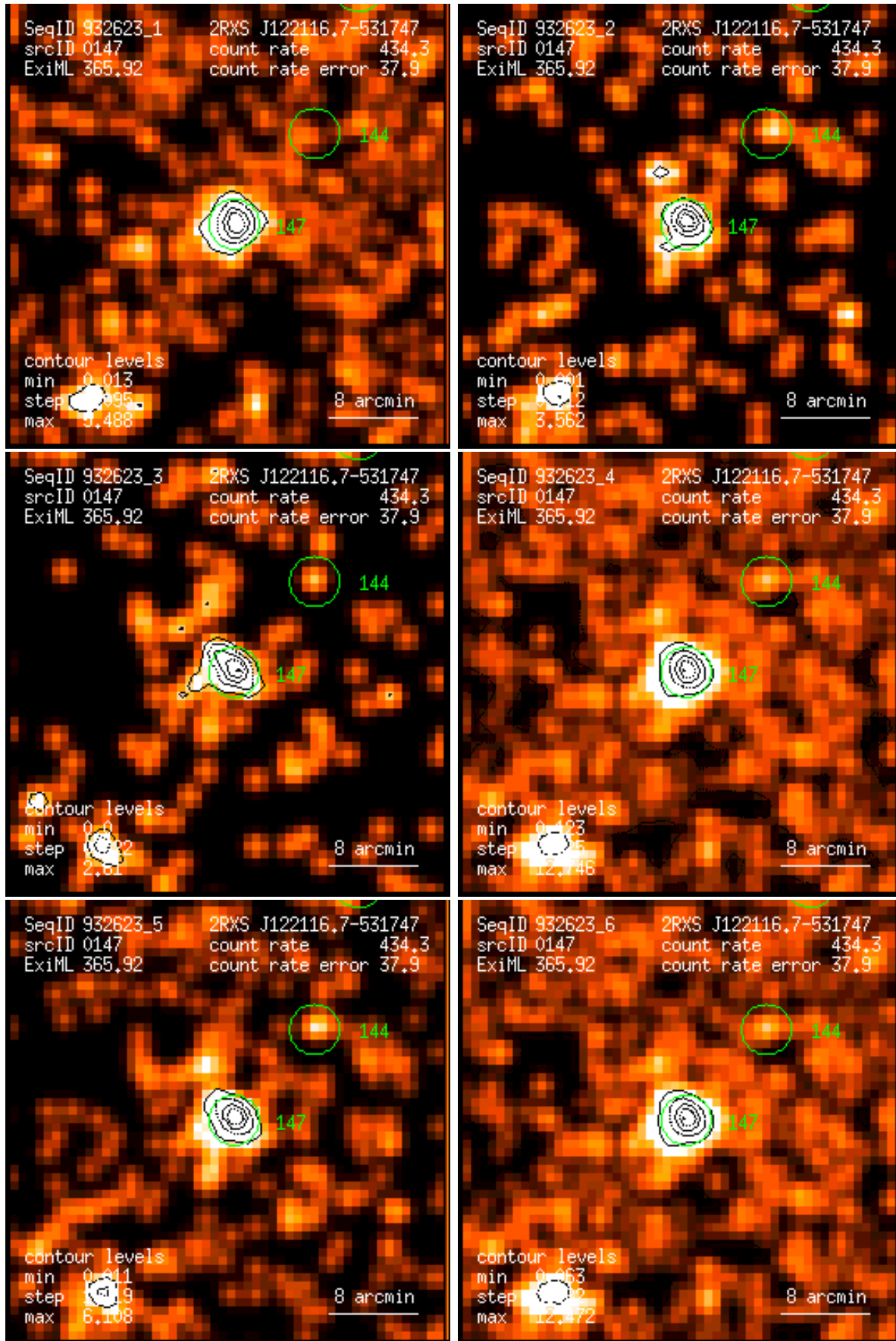
Figure 147: RASS 932623: detection 0147: band rate images, Gaussian filter: (1) PSPC channels 11 – 41, (2) 52 – 90, (3) 91 – 201, (4) 11 – 235, (5) 52 – 201, (6) 11 – 201. Broad band rates in counts/ks. Band rate contour levels in counts/ks/arcmin 2 .
