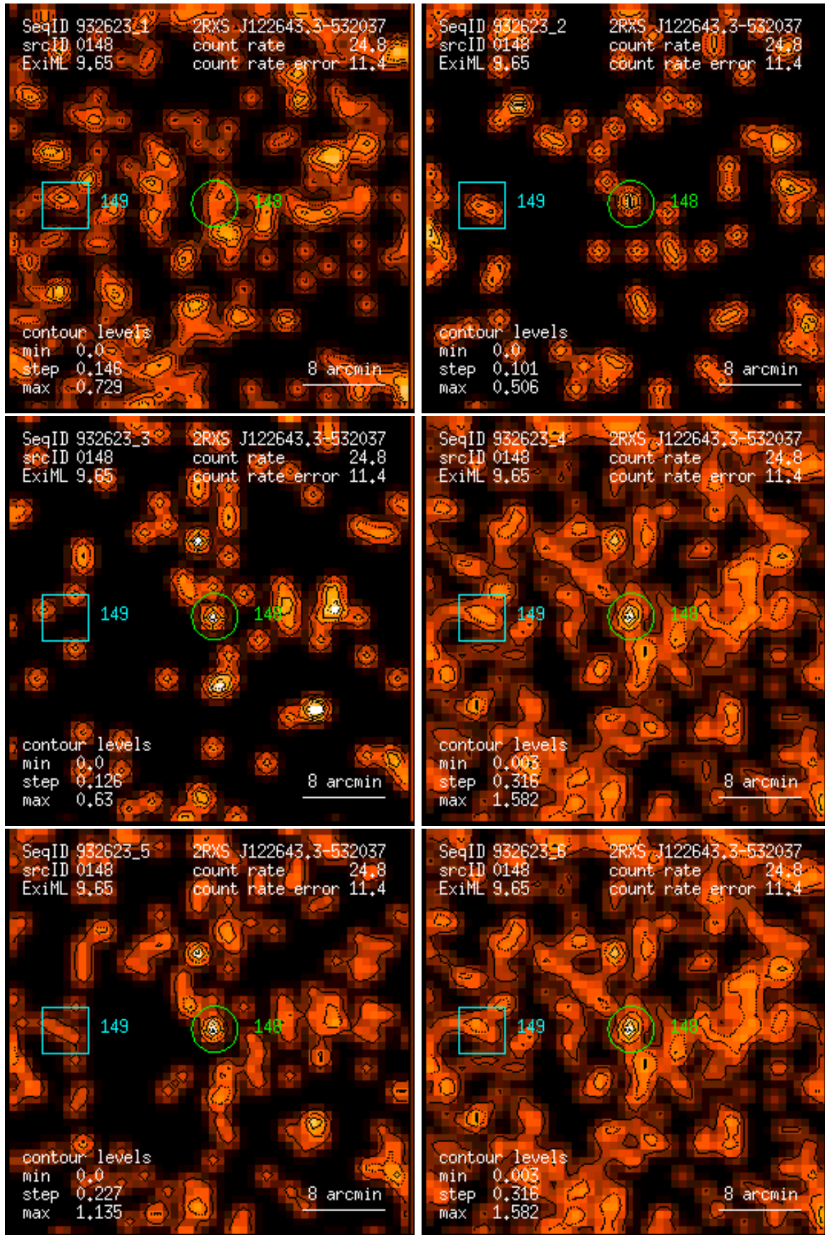
Figure 148: RASS 932623: detection 0148: band rate images, Gaussian filter: (1) PSPC channels 11 – 41, (2) 52 – 90, (3) 91 – 201, (4) 11 – 235, (5) 52 – 201, (6) 11 – 201. Broad band rates in counts/ks. Band rate contour levels in counts/ks/arcmin 2 .
