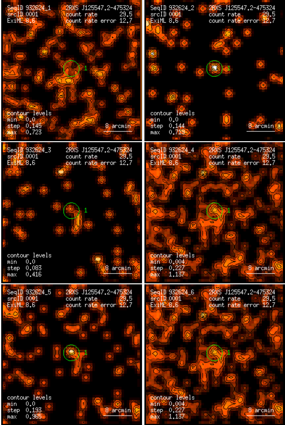
Figure 1: RASS 932624: detection 0001: band rate images, Gaussian filter: (1) PSPC channels 11 – 41, (2) 52 – 90, (3) 91 – 201, (4) 11 – 235, (5) 52 – 201, (6) 11 – 201. Broad band rates in counts/ks. Band rate contour levels in counts/ks/arcmin 2 .
