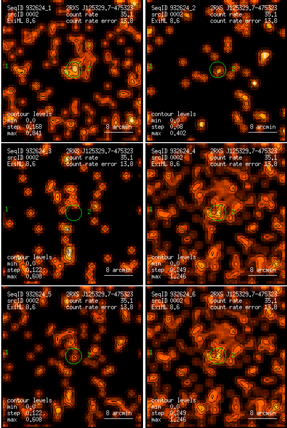
Figure 2: RASS 932624: detection 0002: band rate images, Gaussian filter: (1) PSPC channels 11 – 41, (2) 52 – 90, (3) 91 – 201, (4) 11 – 235, (5) 52 – 201, (6) 11 – 201. Broad band rates in counts/ks. Band rate contour levels in counts/ks/arcmin 2 .
