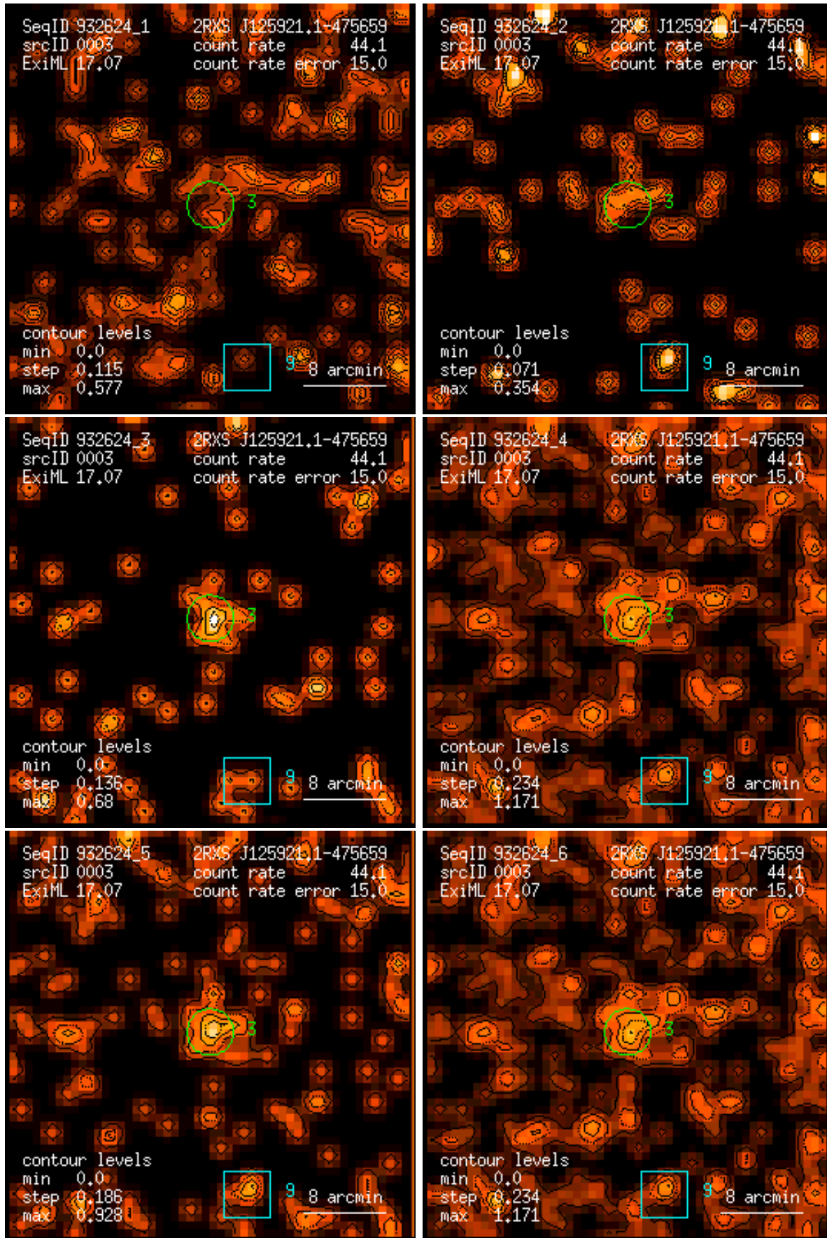
Figure 3: RASS 932624: detection 0003: band rate images, Gaussian filter: (1) PSPC channels 11 – 41, (2) 52 – 90, (3) 91 – 201, (4) 11 – 235, (5) 52 – 201, (6) 11 – 201. Broad band rates in counts/ks. Band rate contour levels in counts/ks/arcmin 2 .
