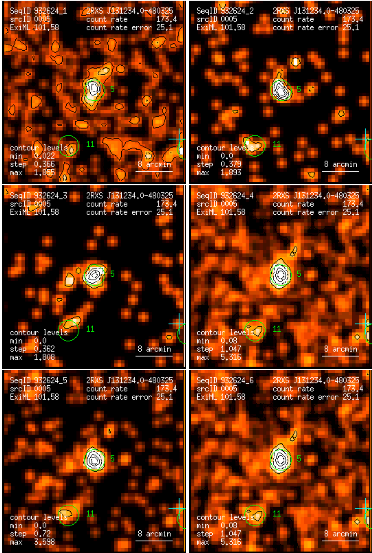
Figure 5: RASS 932624: detection 0005: band rate images, Gaussian filter: (1) PSPC channels 11 – 41, (2) 52 – 90, (3) 91 – 201, (4) 11 – 235, (5) 52 – 201, (6) 11 – 201. Broad band rates in counts/ks. Band rate contour levels in counts/ks/arcmin 2 .
