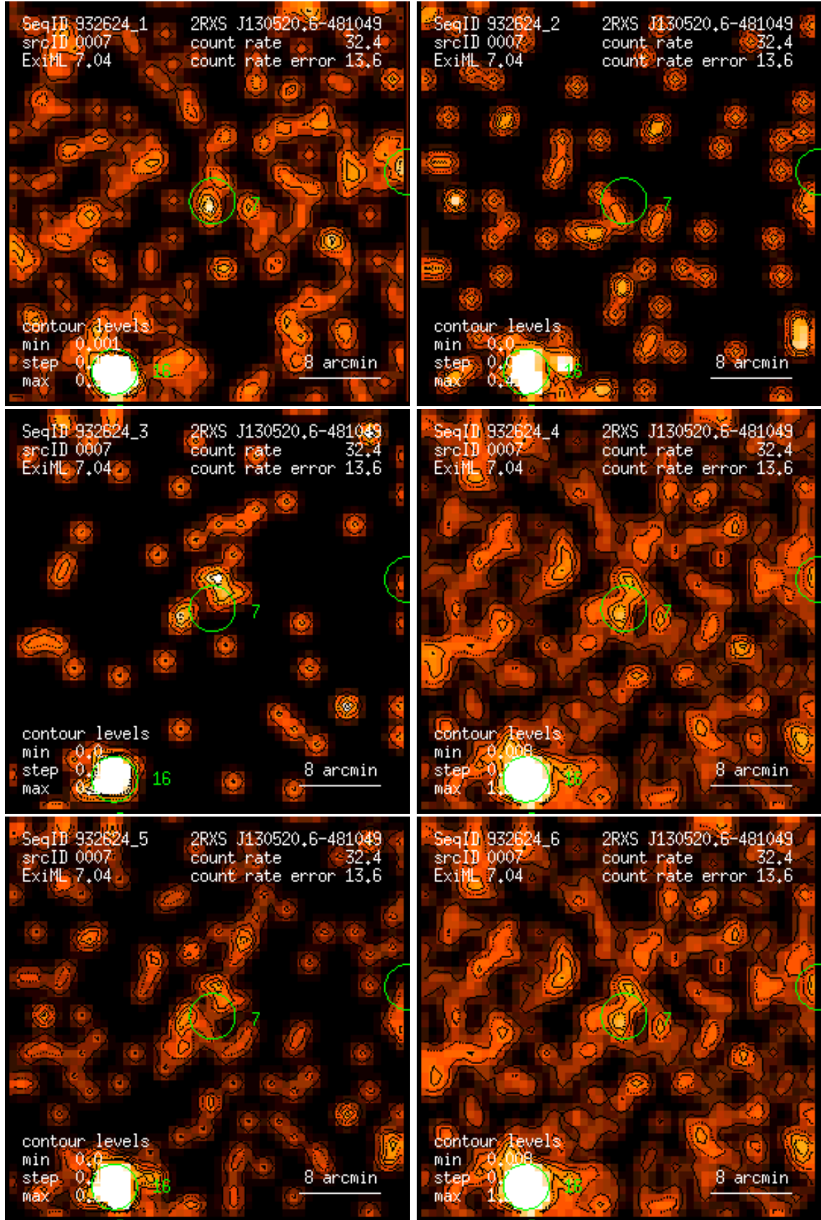
Figure 7: RASS 932624: detection 0007: band rate images, Gaussian filter: (1) PSPC channels 11 – 41, (2) 52 – 90, (3) 91 – 201, (4) 11 – 235, (5) 52 – 201, (6) 11 – 201. Broad band rates in counts/ks. Band rate contour levels in counts/ks/arcmin 2 .
