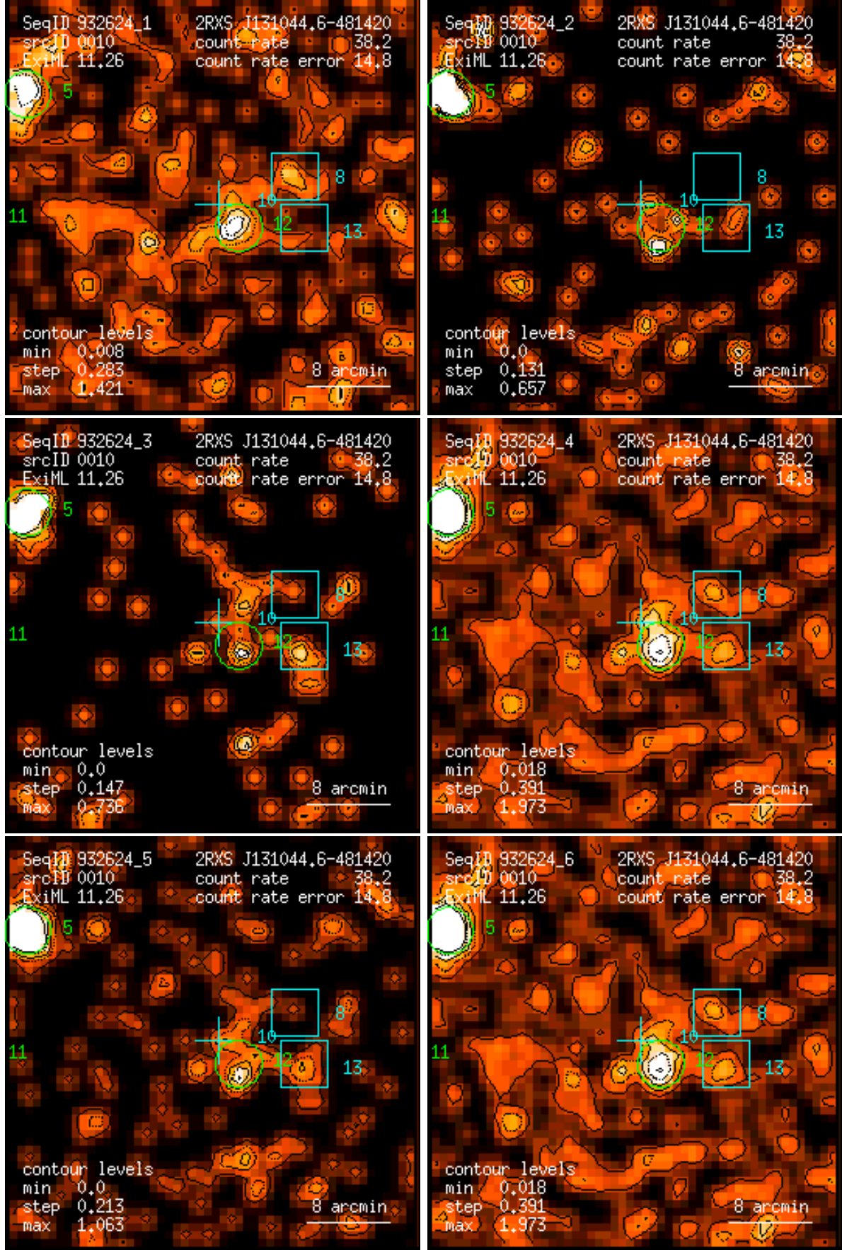
Figure 10: RASS 932624: detection 0010: band rate images, Gaussian filter: (1) PSPC channels 11 – 41, (2) 52 – 90, (3) 91 – 201, (4) 11 – 235, (5) 52 – 201, (6) 11 – 201. Broad band rates in counts/ks. Band rate contour levels in counts/ks/arcmin 2 .
